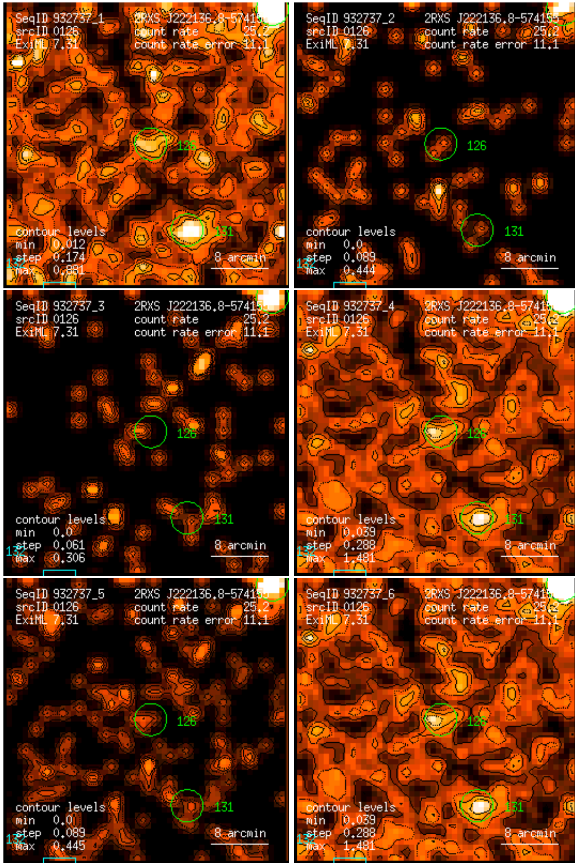
Figure 126: RASS 932737: detection 0126: band rate images, Gaussian filter: (1) PSPC channels 11 – 41, (2) 52 – 90, (3) 91 – 201, (4) 11 – 235, (5) 52 – 201, (6) 11 – 201. Broad band rates in counts/ks. Band rate contour levels in counts/ks/arcmin 2 .
