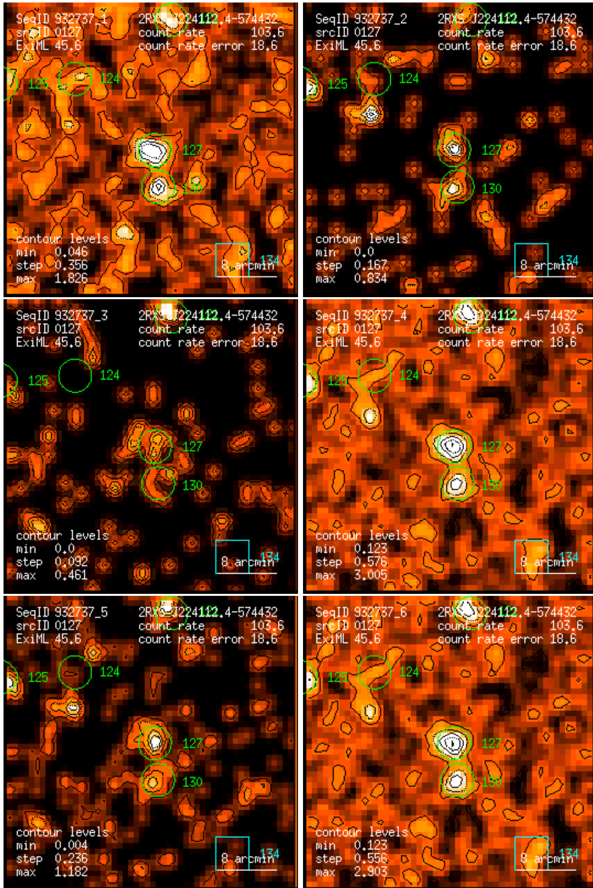
Figure 127: RASS 932737: detection 0127: band rate images, Gaussian filter: (1) PSPC channels 11 – 41, (2) 52 – 90, (3) 91 – 201, (4) 11 – 235, (5) 52 – 201, (6) 11 – 201. Broad band rates in counts/ks. Band rate contour levels in counts/ks/arcmin 2 .
