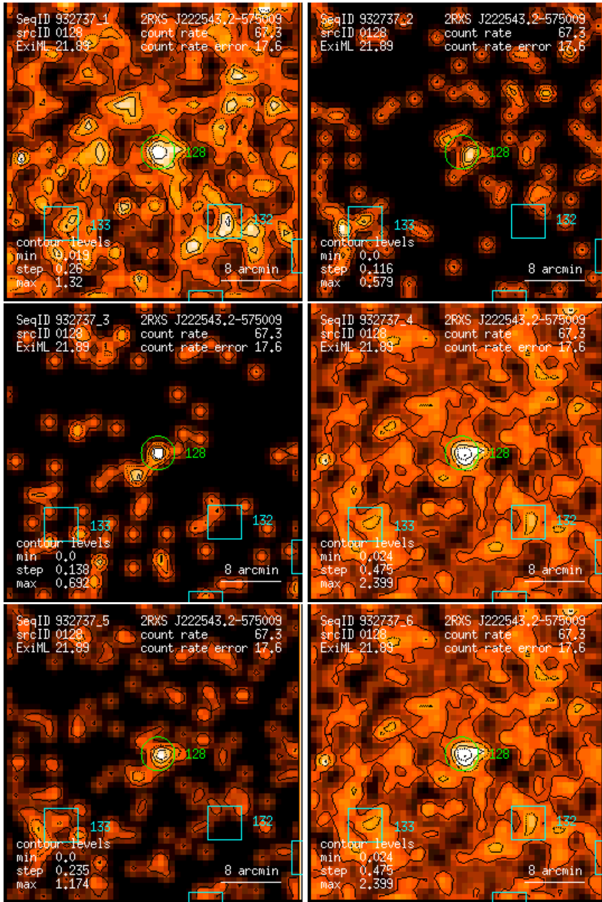
Figure 128: RASS 932737: detection 0128: band rate images, Gaussian filter: (1) PSPC channels 11 – 41, (2) 52 – 90, (3) 91 – 201, (4) 11 – 235, (5) 52 – 201, (6) 11 – 201. Broad band rates in counts/ks. Band rate contour levels in counts/ks/arcmin 2 .
