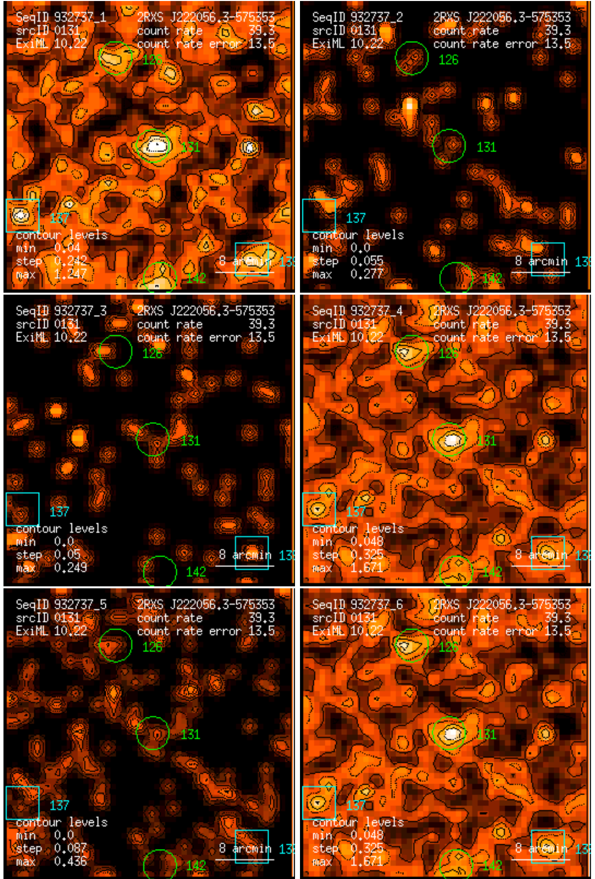
Figure 131: RASS 932737: detection 0131: band rate images, Gaussian filter: (1) PSPC channels 11 – 41, (2) 52 – 90, (3) 91 – 201, (4) 11 – 235, (5) 52 – 201, (6) 11 – 201. Broad band rates in counts/ks. Band rate contour levels in counts/ks/arcmin 2 .
