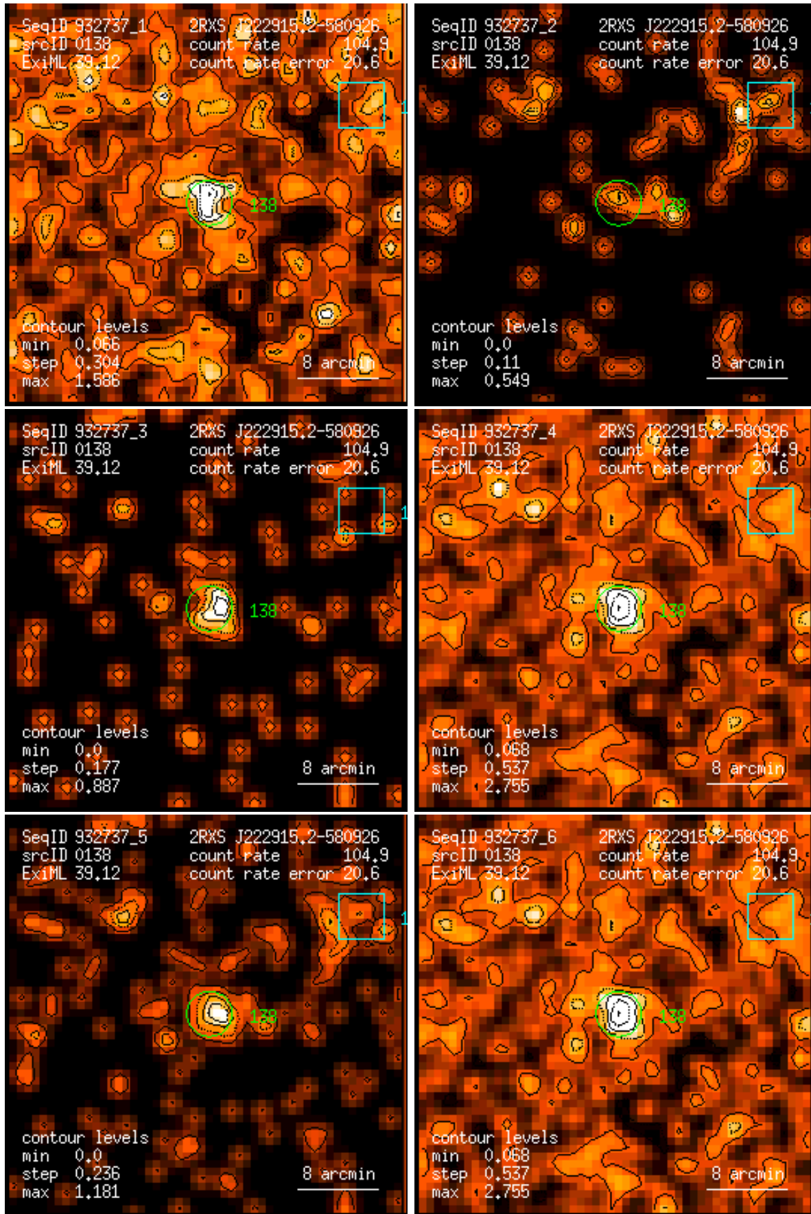
Figure 138: RASS 932737: detection 0138: band rate images, Gaussian filter: (1) PSPC channels 11 – 41, (2) 52 – 90, (3) 91 – 201, (4) 11 – 235, (5) 52 – 201, (6) 11 – 201. Broad band rates in counts/ks. Band rate contour levels in counts/ks/arcmin 2 .
