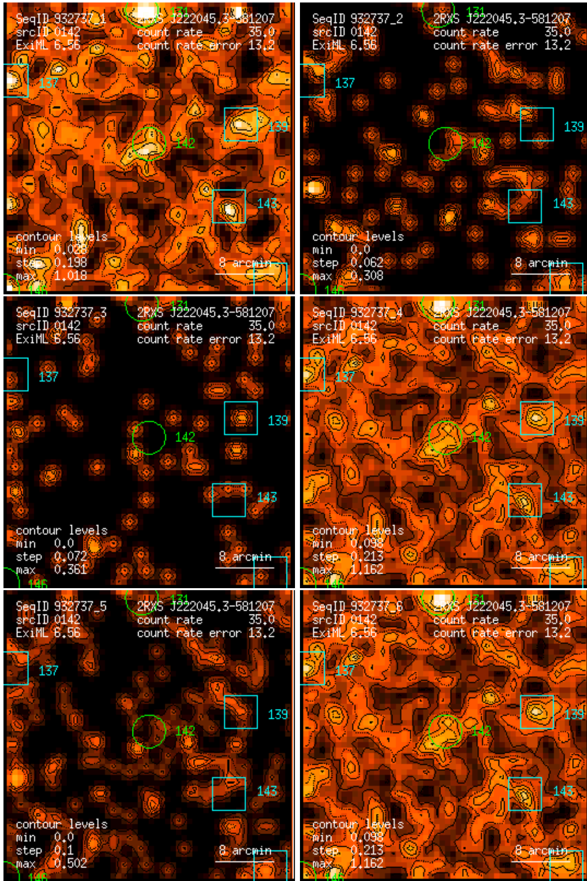
Figure 142: RASS 932737: detection 0142: band rate images, Gaussian filter: (1) PSPC channels 11 – 41, (2) 52 – 90, (3) 91 – 201, (4) 11 – 235, (5) 52 – 201, (6) 11 – 201. Broad band rates in counts/ks. Band rate contour levels in counts/ks/arcmin 2 .
