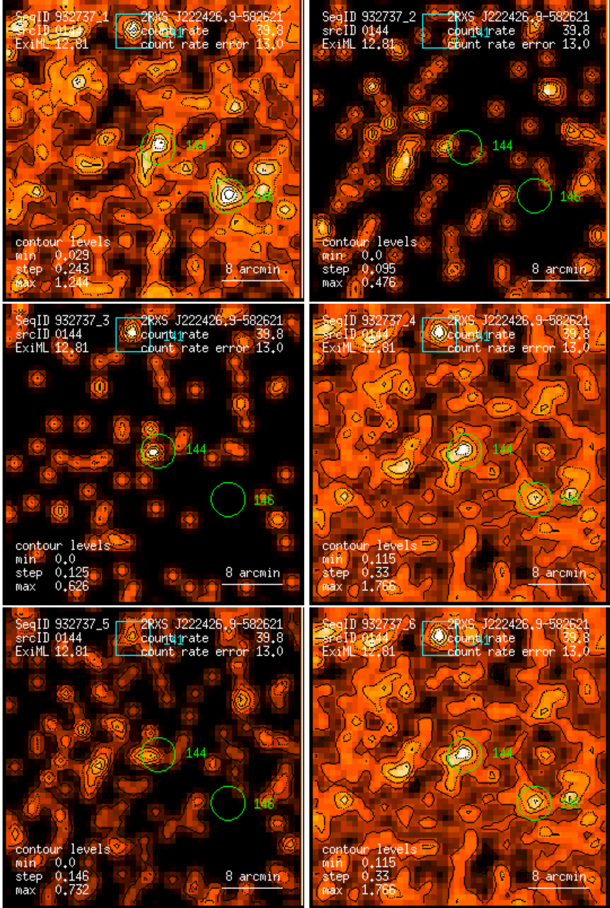
Figure 144: RASS 932737: detection 0144: band rate images, Gaussian filter: (1) PSPC channels 11 – 41, (2) 52 – 90, (3) 91 – 201, (4) 11 – 235, (5) 52 – 201, (6) 11 – 201. Broad band rates in counts/ks. Band rate contour levels in counts/ks/arcmin 2 .
