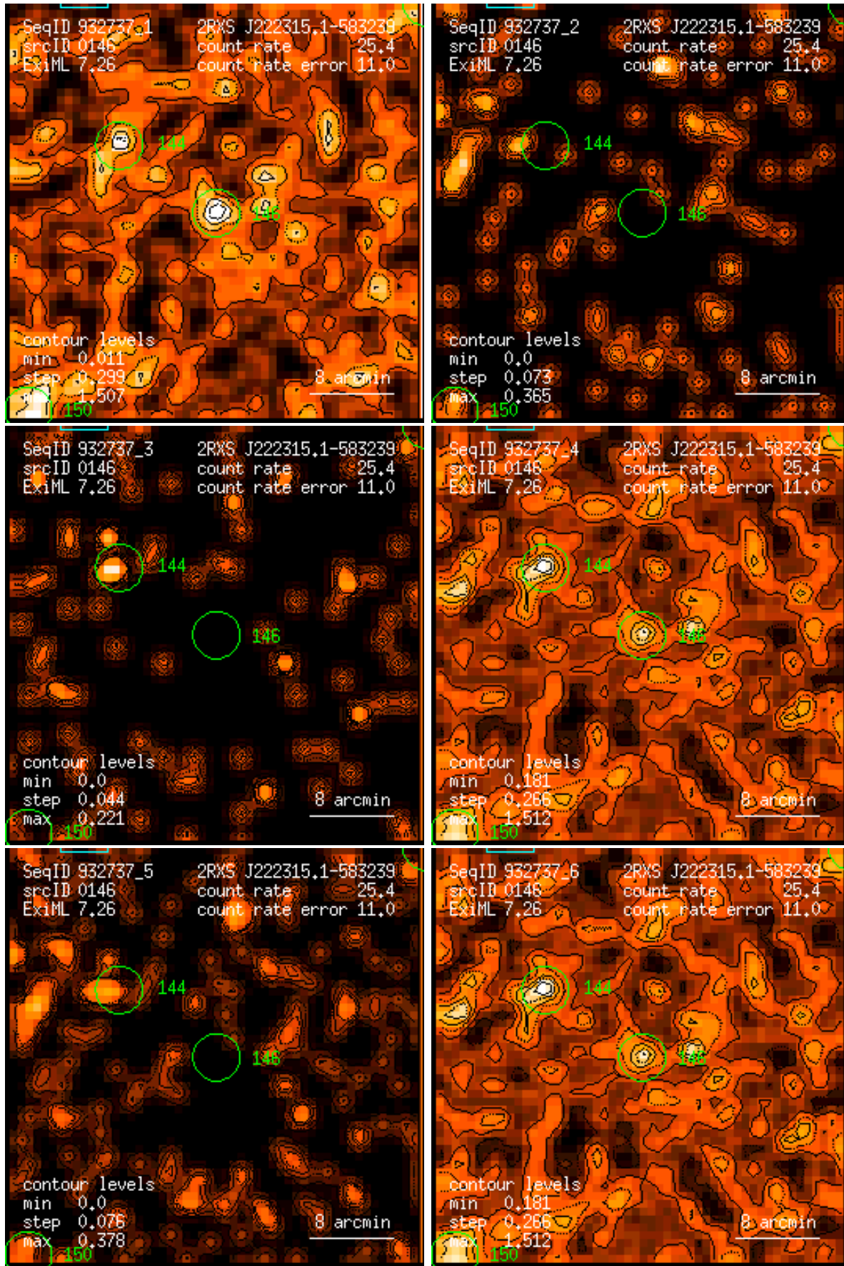
Figure 146: RASS 932737: detection 0146: band rate images, Gaussian filter: (1) PSPC channels 11 – 41, (2) 52 – 90, (3) 91 – 201, (4) 11 – 235, (5) 52 – 201, (6) 11 – 201. Broad band rates in counts/ks. Band rate contour levels in counts/ks/arcmin 2 .
