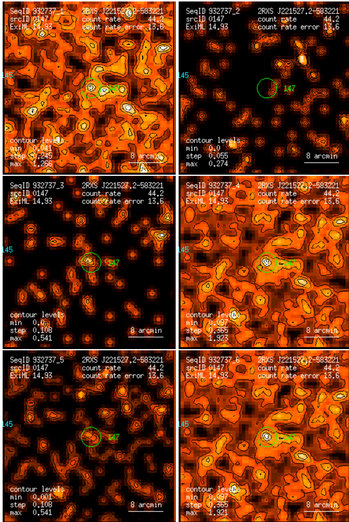
Figure 147: RASS 932737: detection 0147: band rate images, Gaussian filter: (1) PSPC channels 11 – 41, (2) 52 – 90, (3) 91 – 201, (4) 11 – 235, (5) 52 – 201, (6) 11 – 201. Broad band rates in counts/ks. Band rate contour levels in counts/ks/arcmin 2 .
