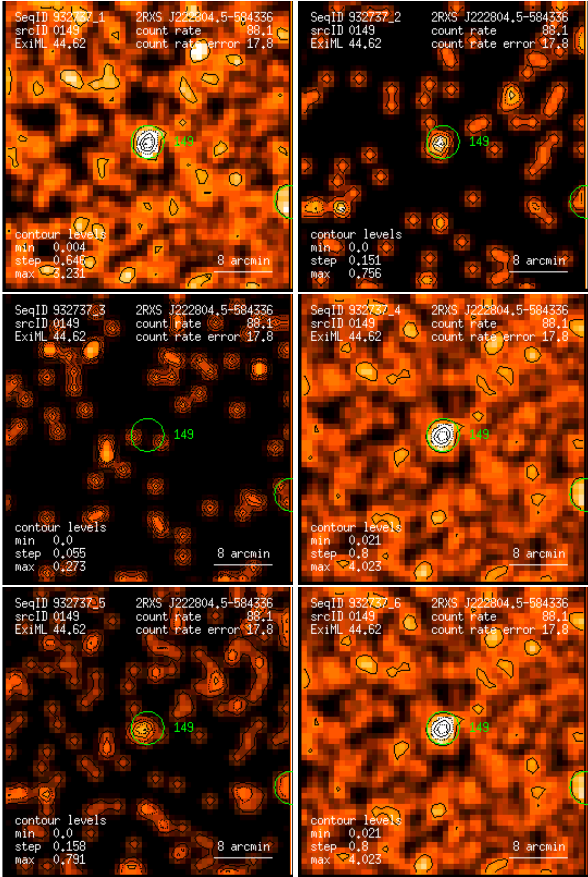
Figure 149: RASS 932737: detection 0149: band rate images, Gaussian filter: (1) PSPC channels 11 – 41, (2) 52 – 90, (3) 91 – 201, (4) 11 – 235, (5) 52 – 201, (6) 11 – 201. Broad band rates in counts/ks. Band rate contour levels in counts/ks/arcmin 2 .
