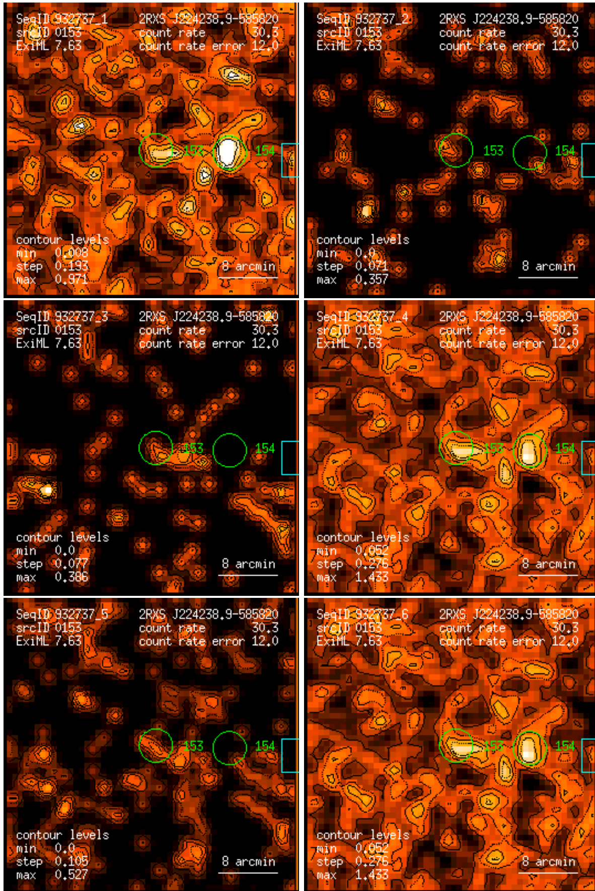
Figure 153: RASS 932737: detection 0153: band rate images, Gaussian filter: (1) PSPC channels 11 – 41, (2) 52 – 90, (3) 91 – 201, (4) 11 – 235, (5) 52 – 201, (6) 11 – 201. Broad band rates in counts/ks. Band rate contour levels in counts/ks/arcmin 2 .
