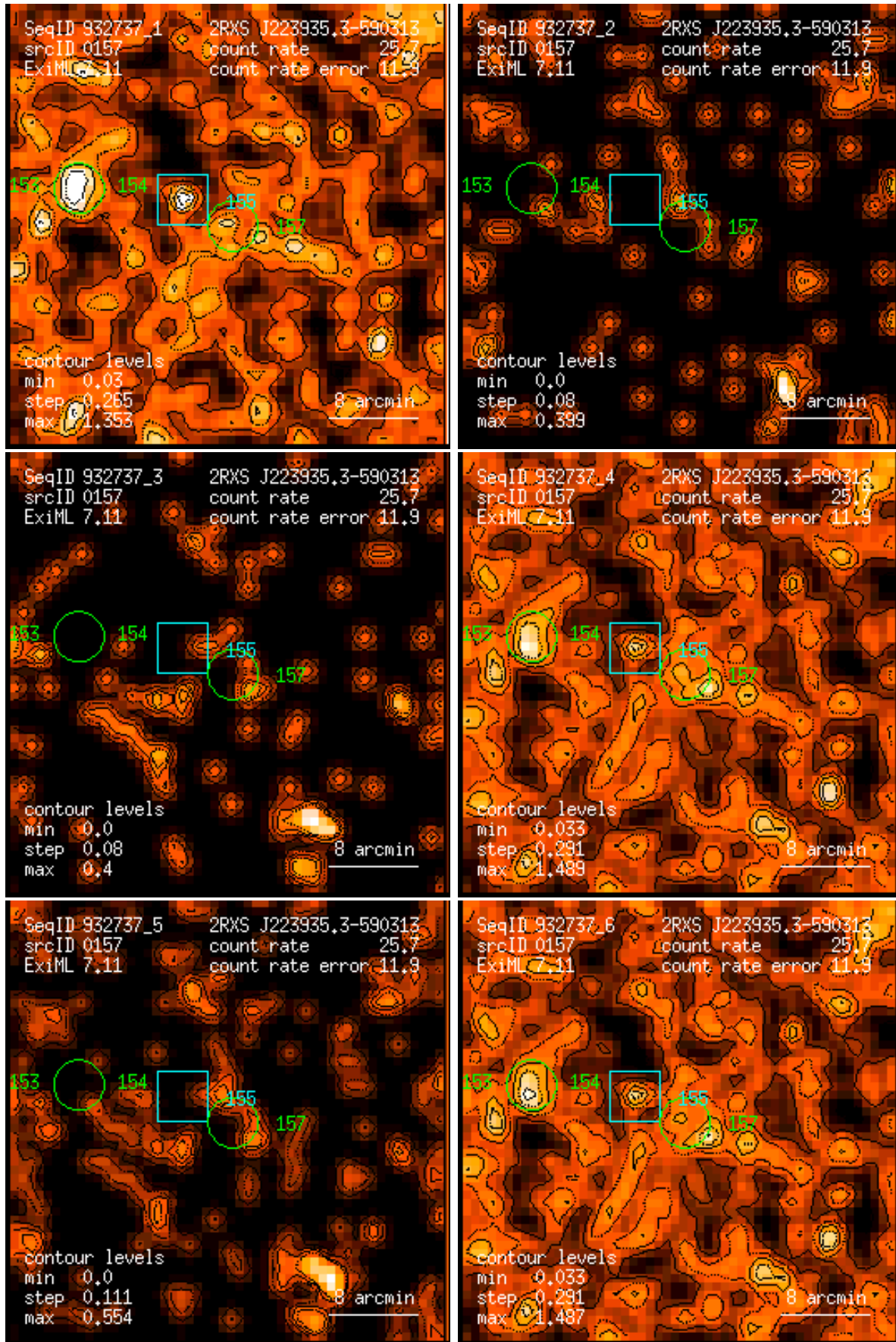
Figure 157: RASS 932737: detection 0157: band rate images, Gaussian filter: (1) PSPC channels 11 – 41, (2) 52 – 90, (3) 91 – 201, (4) 11 – 235, (5) 52 – 201, (6) 11 – 201. Broad band rates in counts/ks. Band rate contour levels in counts/ks/arcmin 2 .
