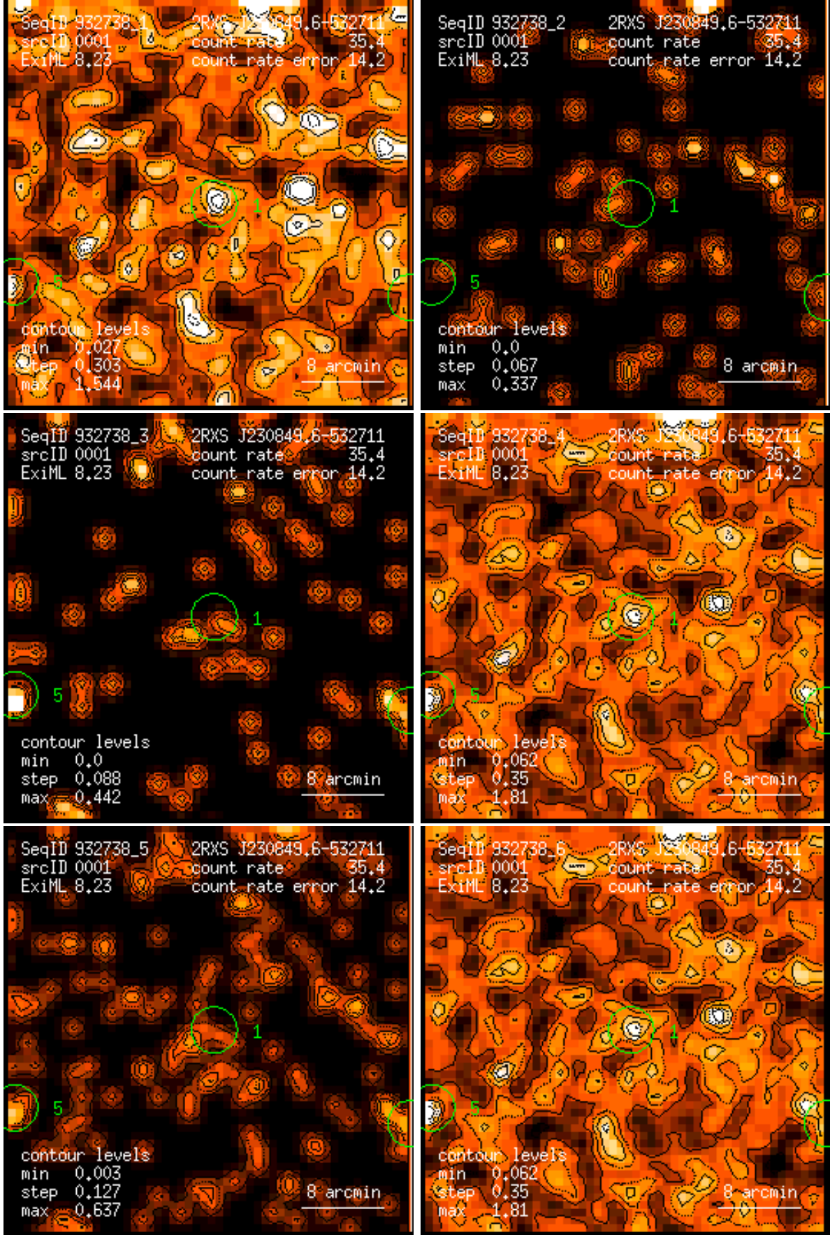
Figure 1: RASS 932738: detection 0001: band rate images, Gaussian filter: (1) PSPC channels 11 – 41, (2) 52 – 90, (3) 91 – 201, (4) 11 – 235, (5) 52 – 201, (6) 11 – 201. Broad band rates in counts/ks. Band rate contour levels in counts/ks/arcmin 2 .
