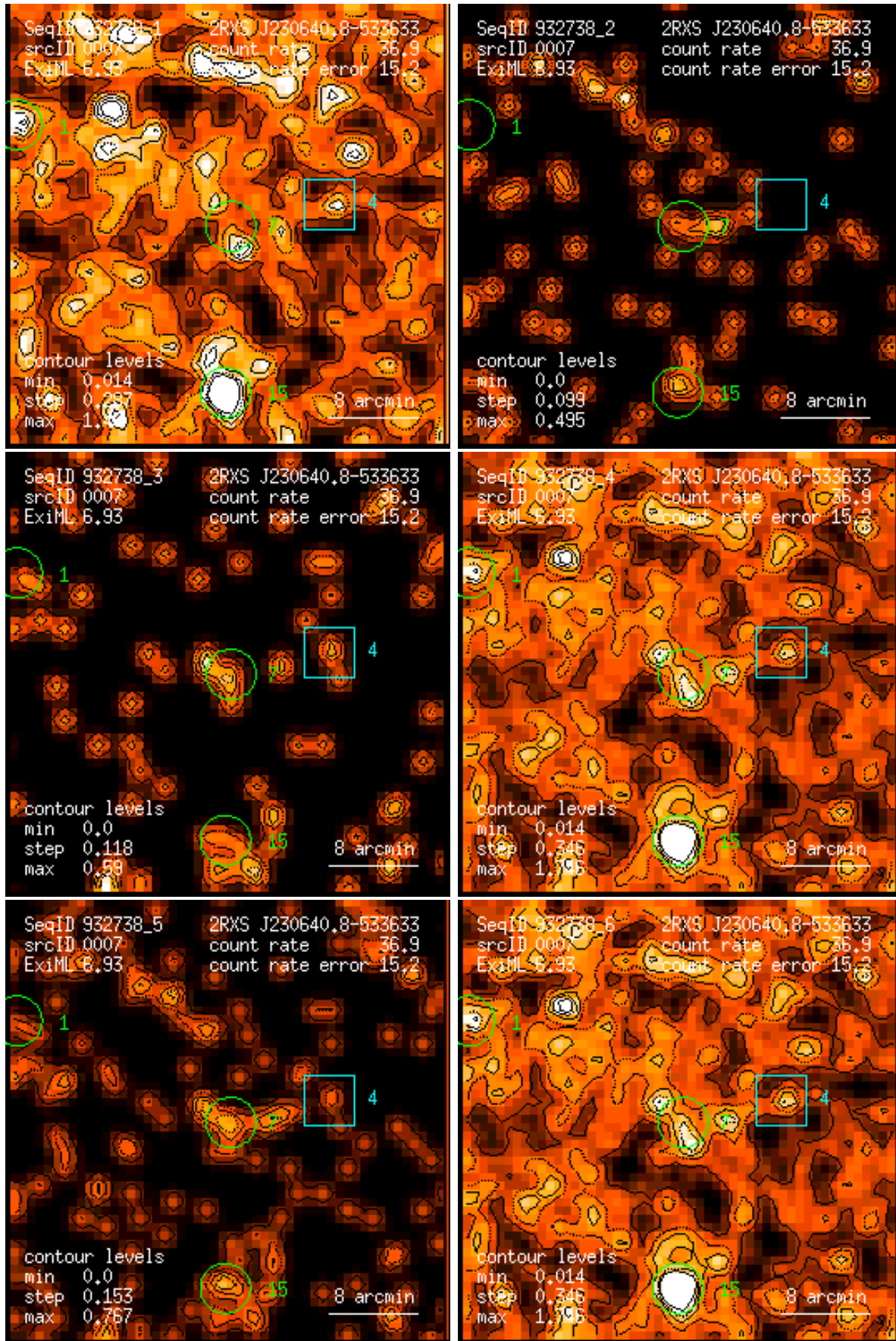
Figure 7: RASS 932738: detection 0007: band rate images, Gaussian filter: (1) PSPC channels 11 – 41, (2) 52 – 90, (3) 91 – 201, (4) 11 – 235, (5) 52 – 201, (6) 11 – 201. Broad band rates in counts/ks. Band rate contour levels in counts/ks/arcmin 2 .
