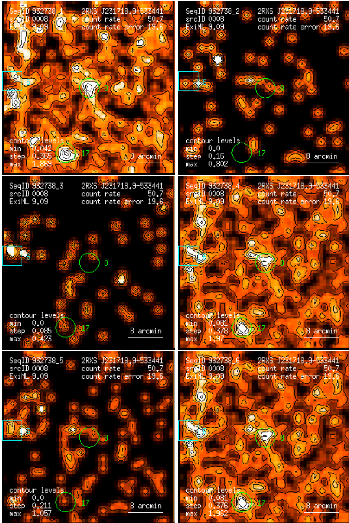
Figure 8: RASS 932738: detection 0008: band rate images, Gaussian filter: (1) PSPC channels 11 – 41, (2) 52 – 90, (3) 91 – 201, (4) 11 – 235, (5) 52 – 201, (6) 11 – 201. Broad band rates in counts/ks. Band rate contour levels in counts/ks/arcmin 2 .
