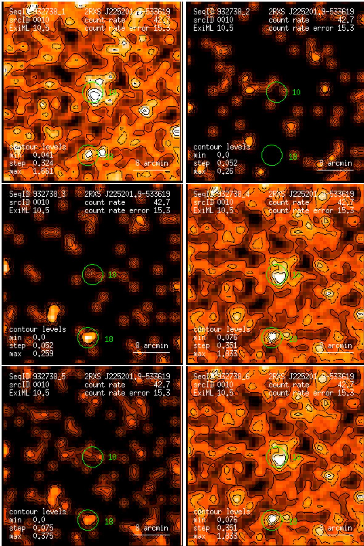
Figure 10: RASS 932738: detection 0010: band rate images, Gaussian filter: (1) PSPC channels 11 – 41, (2) 52 – 90, (3) 91 – 201, (4) 11 – 235, (5) 52 – 201, (6) 11 – 201. Broad band rates in counts/ks. Band rate contour levels in counts/ks/arcmin 2 .
