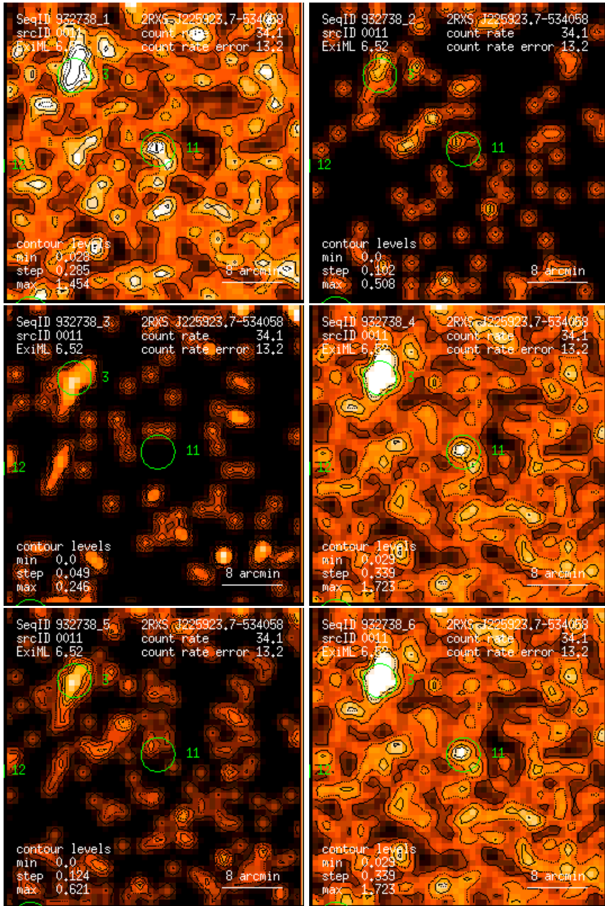
Figure 11: RASS 932738: detection 0011: band rate images, Gaussian filter: (1) PSPC channels 11 – 41, (2) 52 – 90, (3) 91 – 201, (4) 11 – 235, (5) 52 – 201, (6) 11 – 201. Broad band rates in counts/ks. Band rate contour levels in counts/ks/arcmin 2 .
