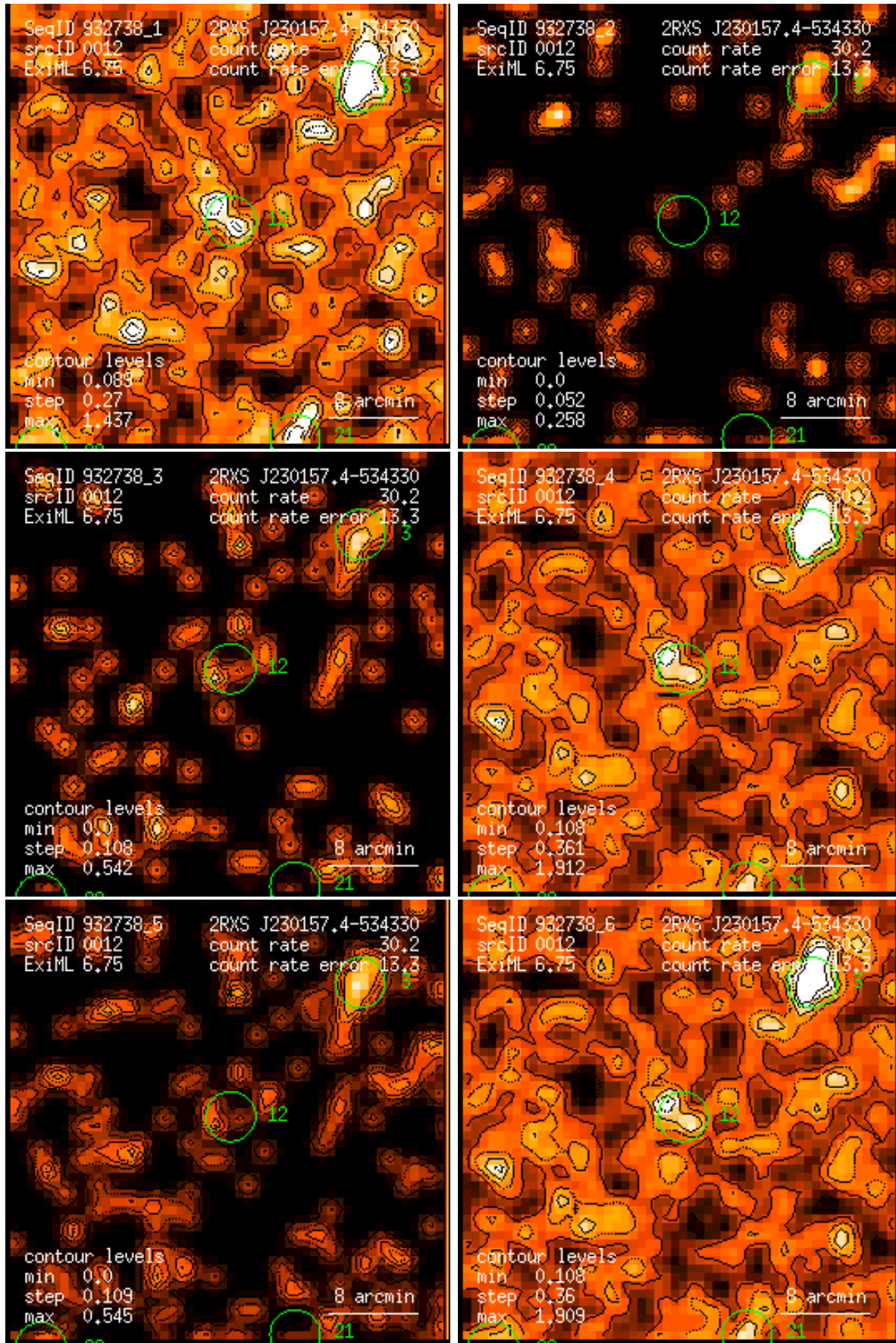
Figure 12: RASS 932738: detection 0012: band rate images, Gaussian filter: (1) PSPC channels 11 – 41, (2) 52 – 90, (3) 91 – 201, (4) 11 – 235, (5) 52 – 201, (6) 11 – 201. Broad band rates in counts/ks. Band rate contour levels in counts/ks/arcmin 2 .
