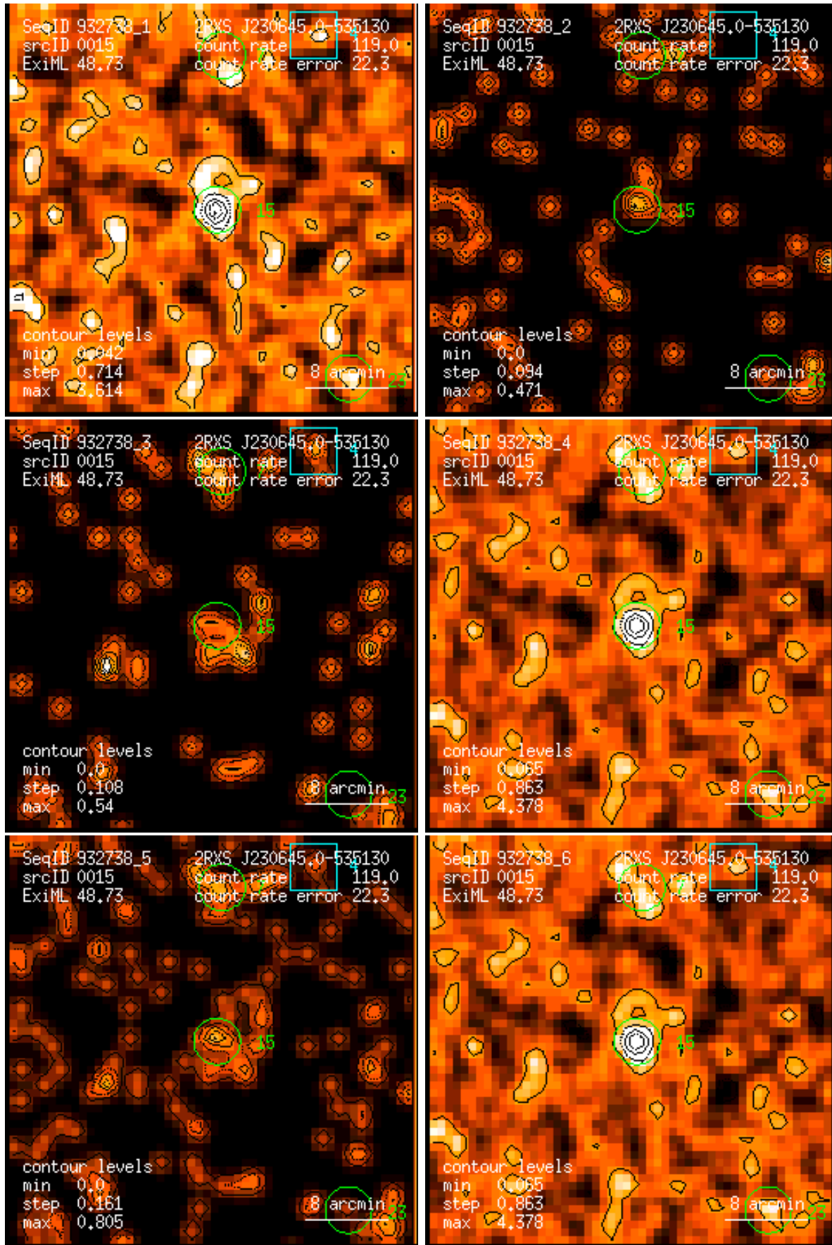
Figure 15: RASS 932738: detection 0015: band rate images, Gaussian filter: (1) PSPC channels 11 – 41, (2) 52 – 90, (3) 91 – 201, (4) 11 – 235, (5) 52 – 201, (6) 11 – 201. Broad band rates in counts/ks. Band rate contour levels in counts/ks/arcmin 2 .
