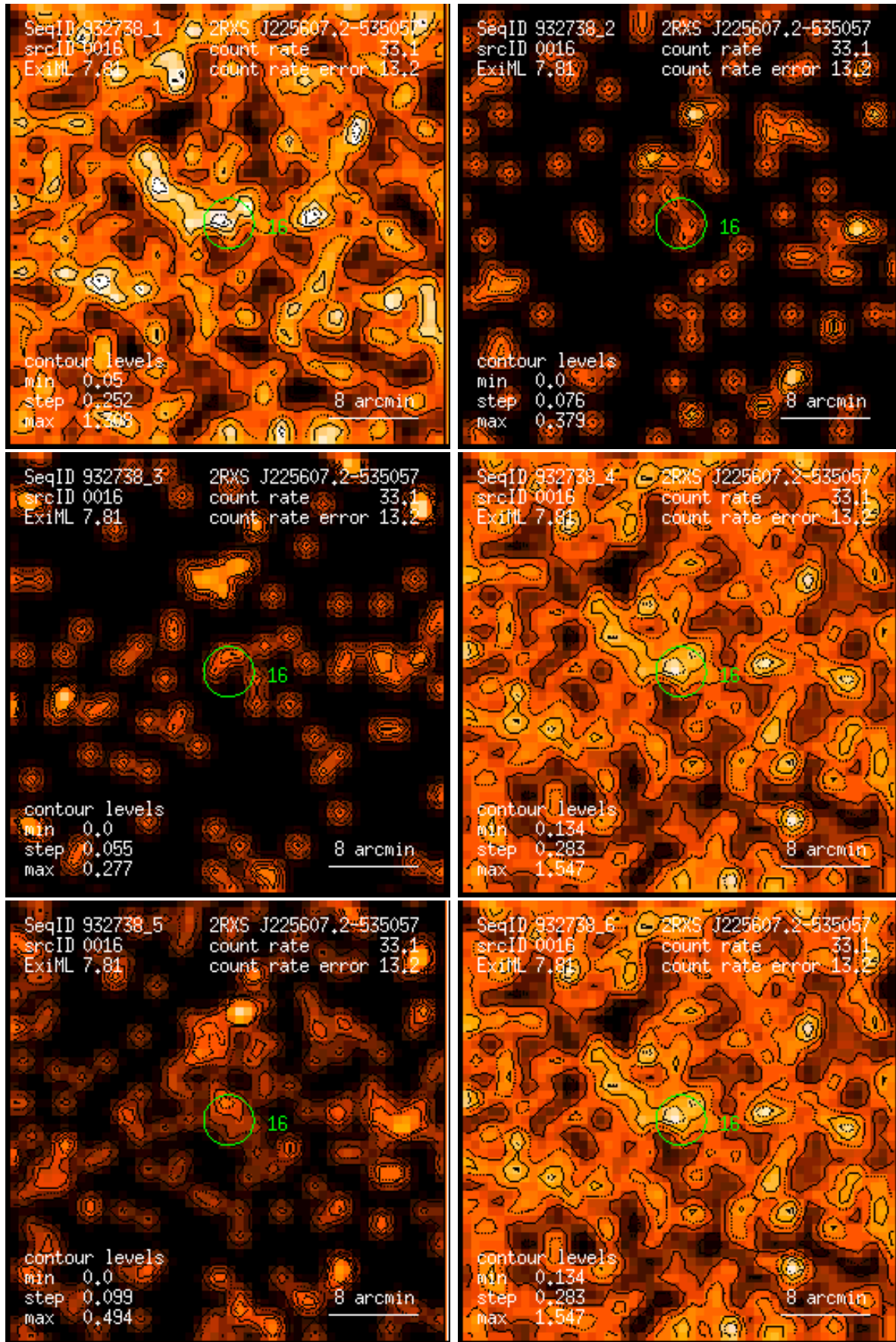
Figure 16: RASS 932738: detection 0016: band rate images, Gaussian filter: (1) PSPC channels 11 – 41, (2) 52 – 90, (3) 91 – 201, (4) 11 – 235, (5) 52 – 201, (6) 11 – 201. Broad band rates in counts/ks. Band rate contour levels in counts/ks/arcmin 2 .
