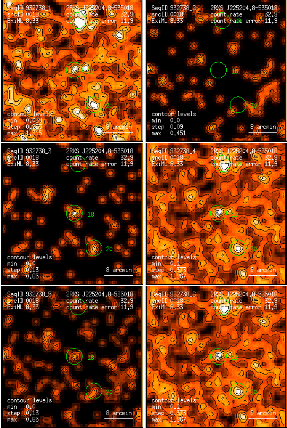
Figure 18: RASS 932738: detection 0018: band rate images, Gaussian filter: (1) PSPC channels 11 – 41, (2) 52 – 90, (3) 91 – 201, (4) 11 – 235, (5) 52 – 201, (6) 11 – 201. Broad band rates in counts/ks. Band rate contour levels in counts/ks/arcmin 2 .
