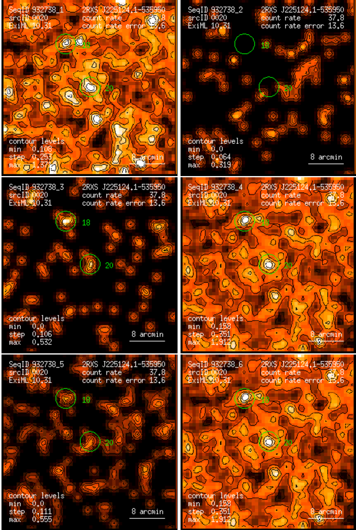
Figure 20: RASS 932738: detection 0020: band rate images, Gaussian filter: (1) PSPC channels 11 – 41, (2) 52 – 90, (3) 91 – 201, (4) 11 – 235, (5) 52 – 201, (6) 11 – 201. Broad band rates in counts/ks. Band rate contour levels in counts/ks/arcmin 2 .
