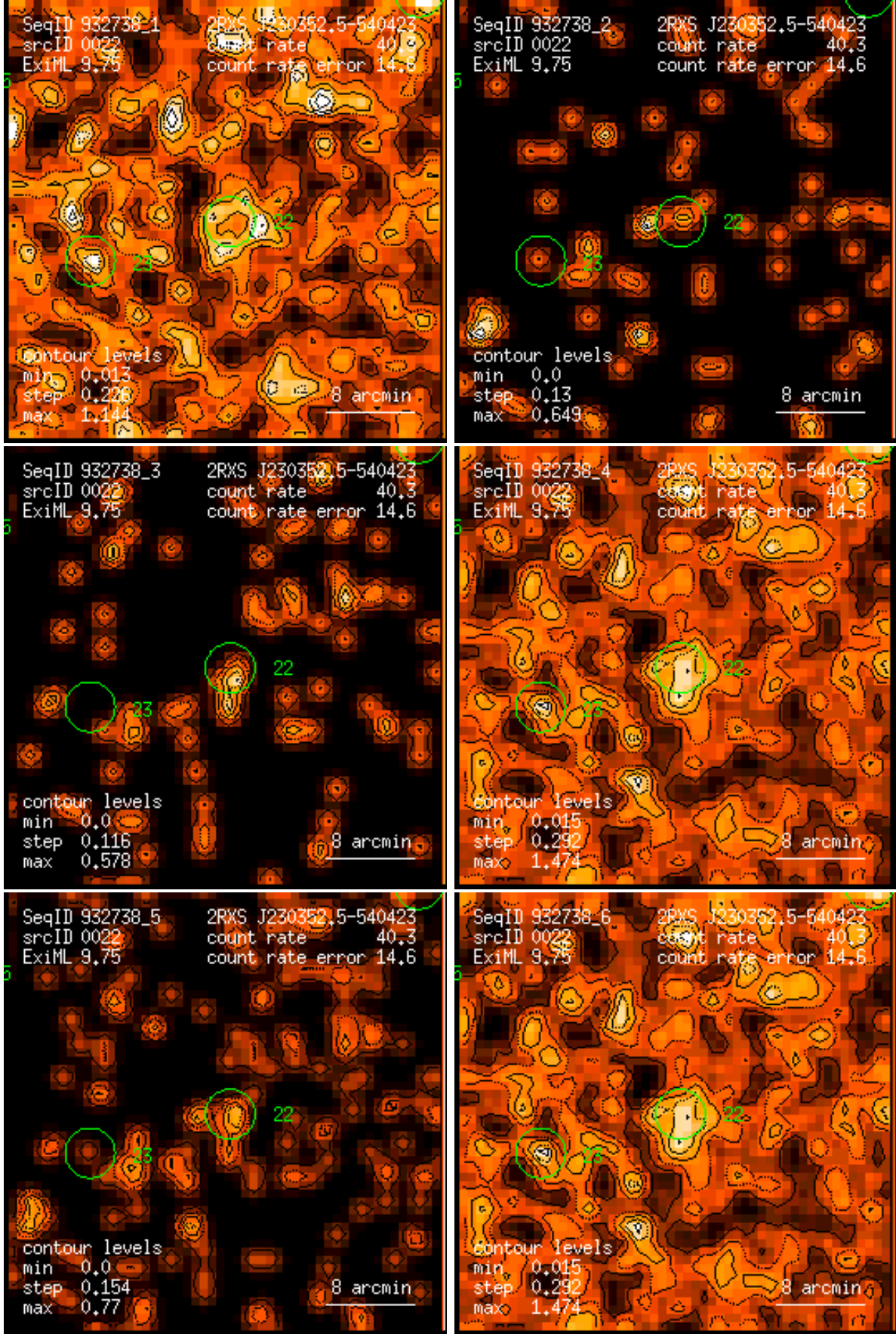
Figure 22: RASS 932738: detection 0022: band rate images, Gaussian filter: (1) PSPC channels 11 – 41, (2) 52 – 90, (3) 91 – 201, (4) 11 – 235, (5) 52 – 201, (6) 11 – 201. Broad band rates in counts/ks. Band rate contour levels in counts/ks/arcmin 2 .
