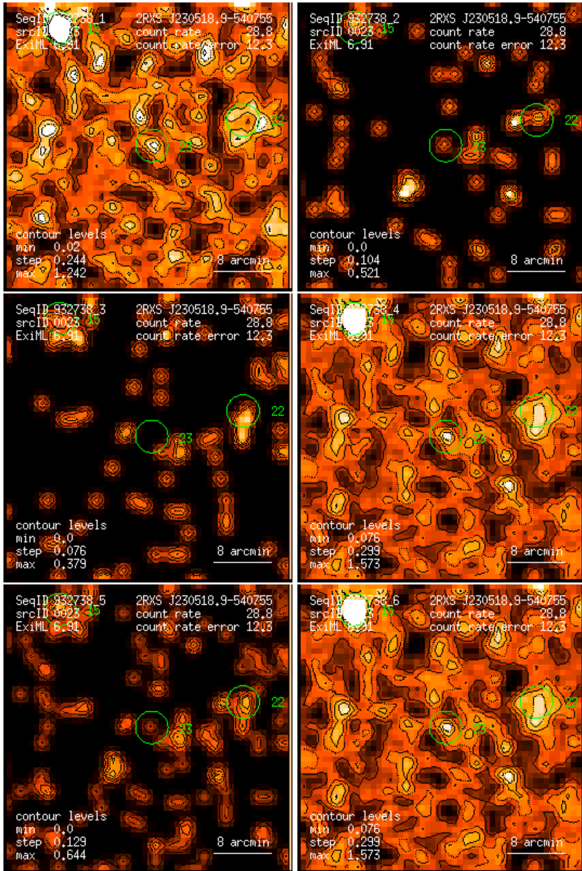
Figure 23: RASS 932738: detection 0023: band rate images, Gaussian filter: (1) PSPC channels 11 – 41, (2) 52 – 90, (3) 91 – 201, (4) 11 – 235, (5) 52 – 201, (6) 11 – 201. Broad band rates in counts/ks. Band rate contour levels in counts/ks/arcmin 2 .
