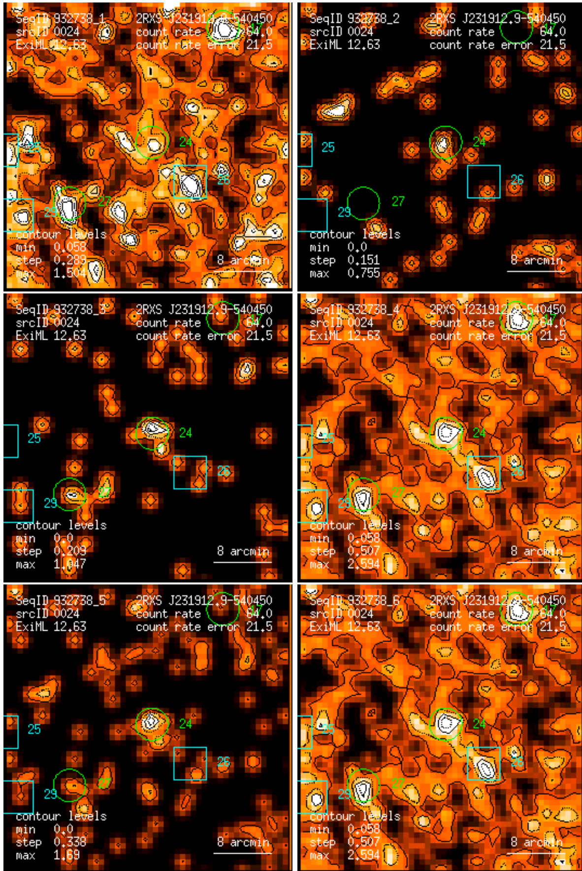
Figure 24: RASS 932738: detection 0024: band rate images, Gaussian filter: (1) PSPC channels 11 – 41, (2) 52 – 90, (3) 91 – 201, (4) 11 – 235, (5) 52 – 201, (6) 11 – 201. Broad band rates in counts/ks. Band rate contour levels in counts/ks/arcmin 2 .
