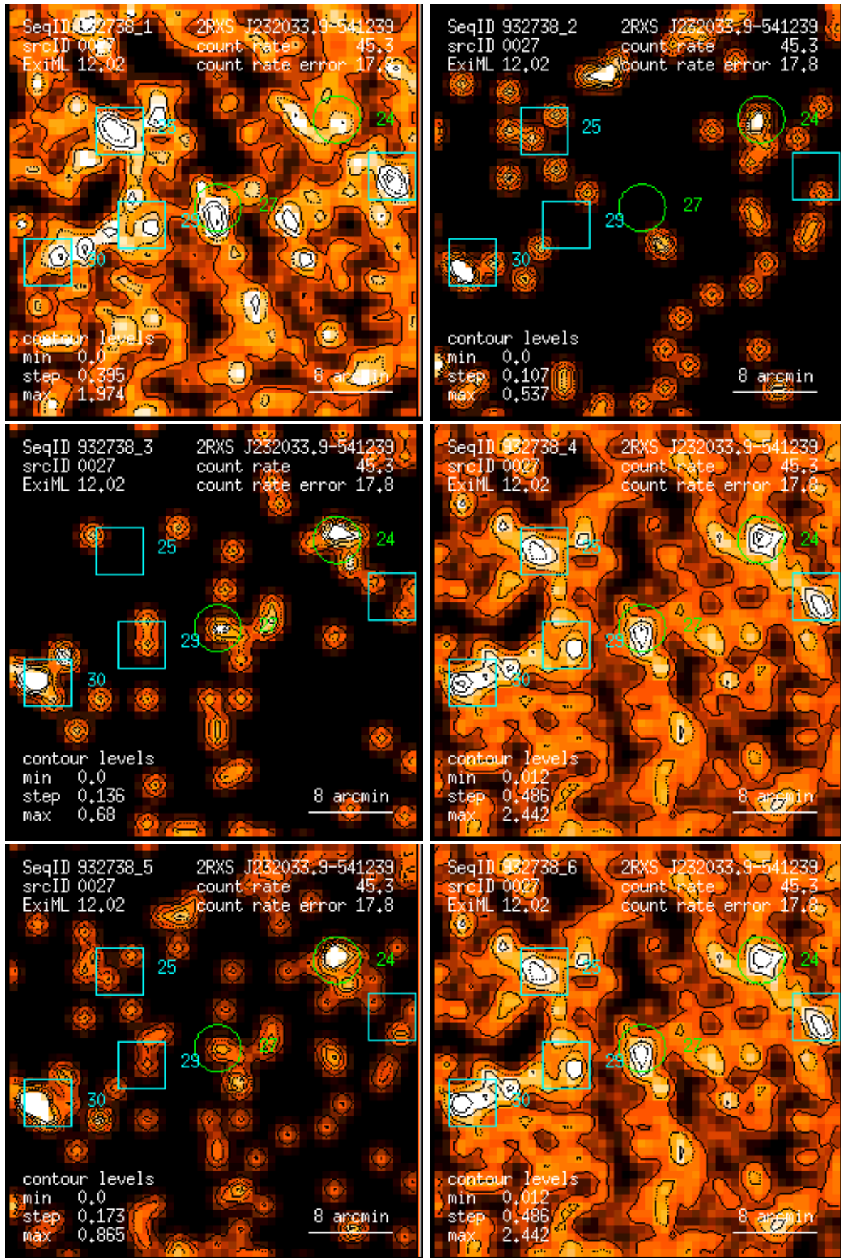
Figure 27: RASS 932738: detection 0027: band rate images, Gaussian filter: (1) PSPC channels 11 – 41, (2) 52 – 90, (3) 91 – 201, (4) 11 – 235, (5) 52 – 201, (6) 11 – 201. Broad band rates in counts/ks. Band rate contour levels in counts/ks/arcmin 2 .
