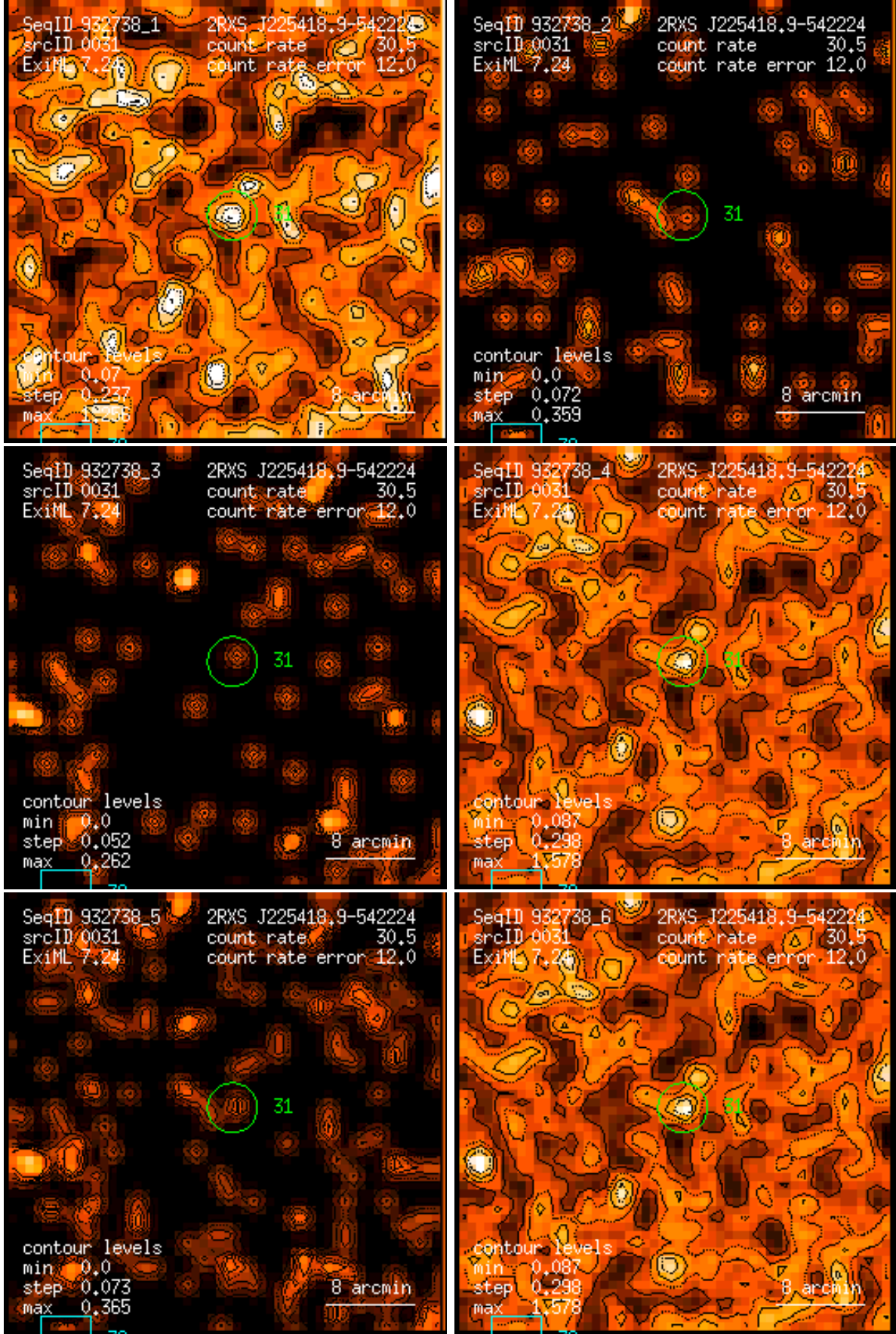
Figure 31: RASS 932738: detection 0031: band rate images, Gaussian filter: (1) PSPC channels 11 – 41, (2) 52 – 90, (3) 91 – 201, (4) 11 – 235, (5) 52 – 201, (6) 11 – 201. Broad band rates in counts/ks. Band rate contour levels in counts/ks/arcmin 2 .
