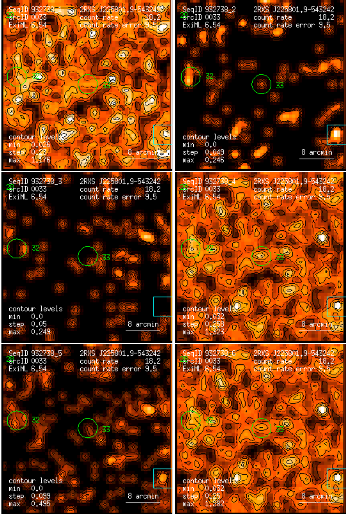
Figure 33: RASS 932738: detection 0033: band rate images, Gaussian filter: (1) PSPC channels 11 – 41, (2) 52 – 90, (3) 91 – 201, (4) 11 – 235, (5) 52 – 201, (6) 11 – 201. Broad band rates in counts/ks. Band rate contour levels in counts/ks/arcmin 2 .
