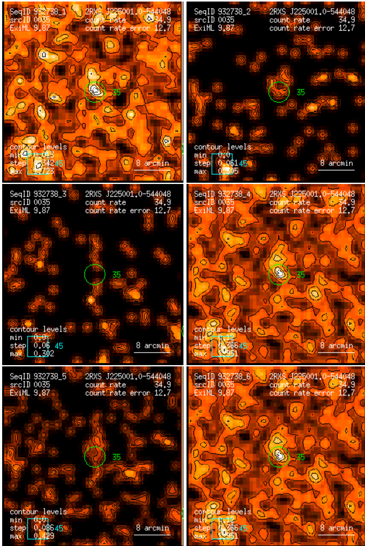
Figure 35: RASS 932738: detection 0035: band rate images, Gaussian filter: (1) PSPC channels 11 – 41, (2) 52 – 90, (3) 91 – 201, (4) 11 – 235, (5) 52 – 201, (6) 11 – 201. Broad band rates in counts/ks. Band rate contour levels in counts/ks/arcmin 2 .
