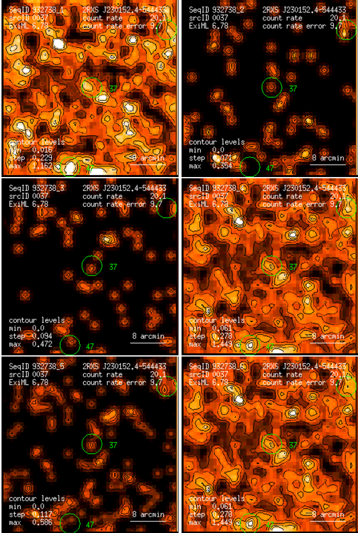
Figure 37: RASS 932738: detection 0037: band rate images, Gaussian filter: (1) PSPC channels 11 – 41, (2) 52 – 90, (3) 91 – 201, (4) 11 – 235, (5) 52 – 201, (6) 11 – 201. Broad band rates in counts/ks. Band rate contour levels in counts/ks/arcmin 2 .
