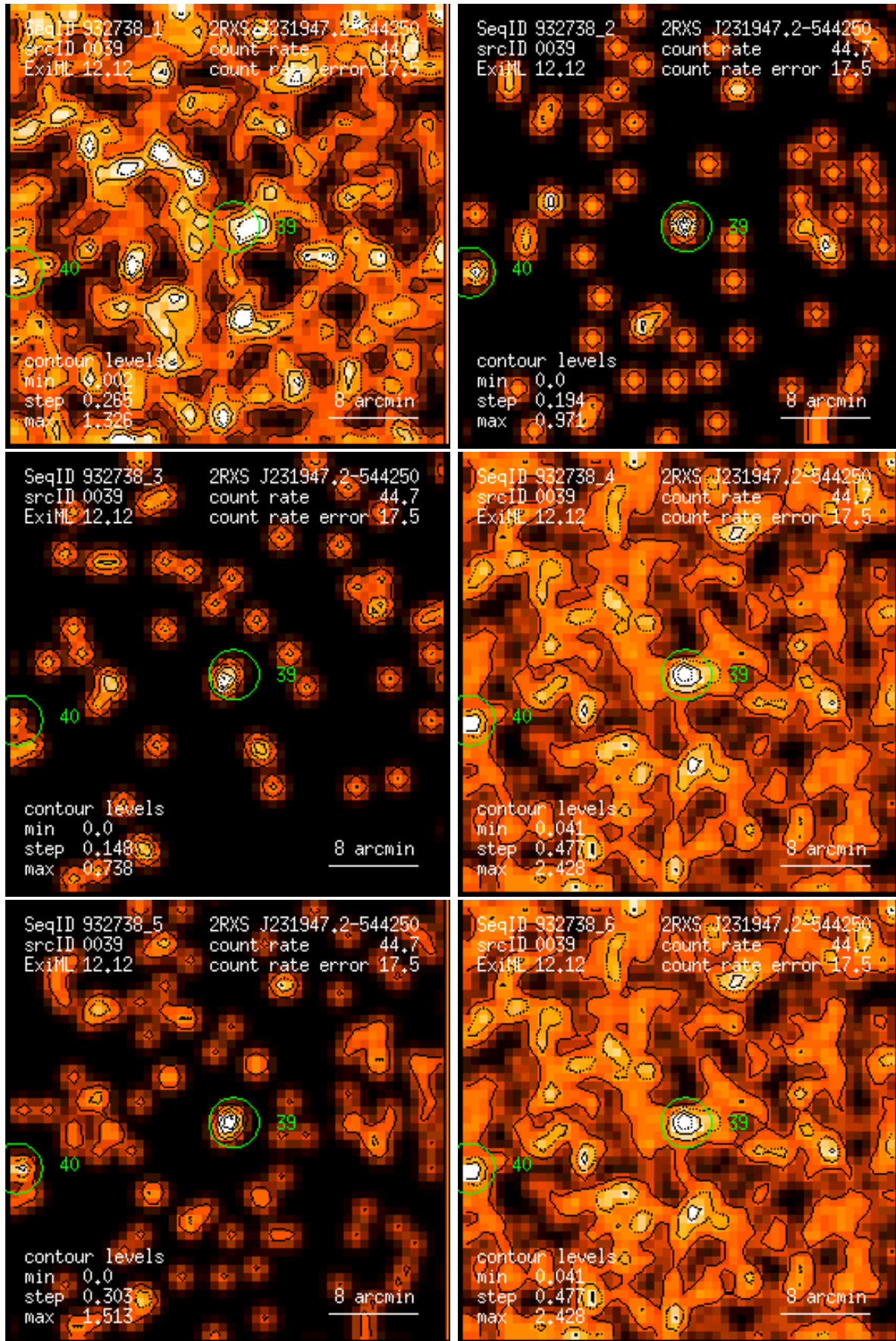
Figure 39: RASS 932738: detection 0039: band rate images, Gaussian filter: (1) PSPC channels 11 – 41, (2) 52 – 90, (3) 91 – 201, (4) 11 – 235, (5) 52 – 201, (6) 11 – 201. Broad band rates in counts/ks. Band rate contour levels in counts/ks/arcmin 2 .
