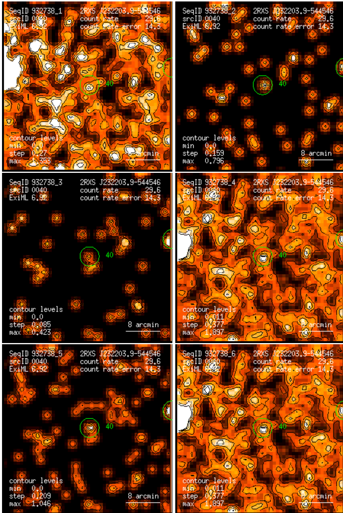
Figure 40: RASS 932738: detection 0040: band rate images, Gaussian filter: (1) PSPC channels 11 – 41, (2) 52 – 90, (3) 91 – 201, (4) 11 – 235, (5) 52 – 201, (6) 11 – 201. Broad band rates in counts/ks. Band rate contour levels in counts/ks/arcmin 2 .
