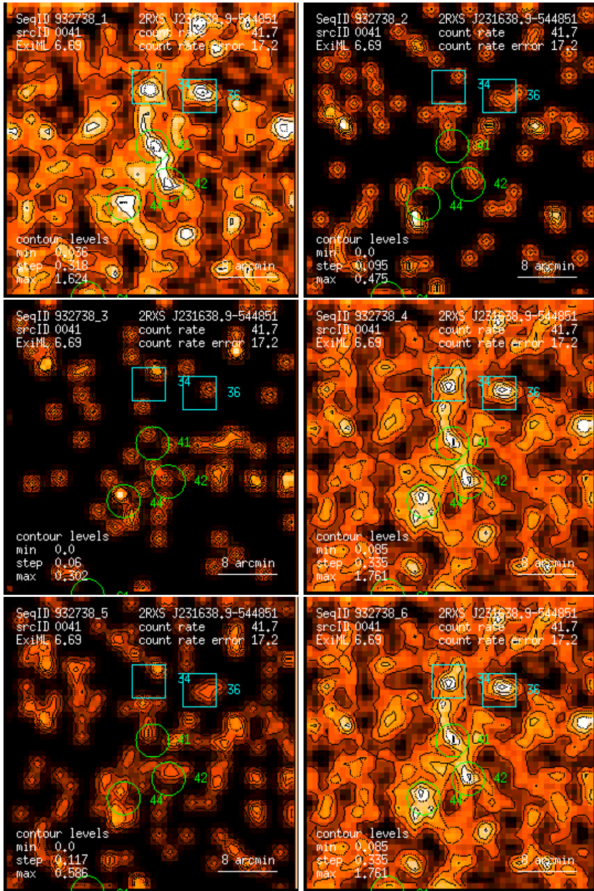
Figure 41: RASS 932738: detection 0041: band rate images, Gaussian filter: (1) PSPC channels 11 – 41, (2) 52 – 90, (3) 91 – 201, (4) 11 – 235, (5) 52 – 201, (6) 11 – 201. Broad band rates in counts/ks. Band rate contour levels in counts/ks/arcmin 2 .
