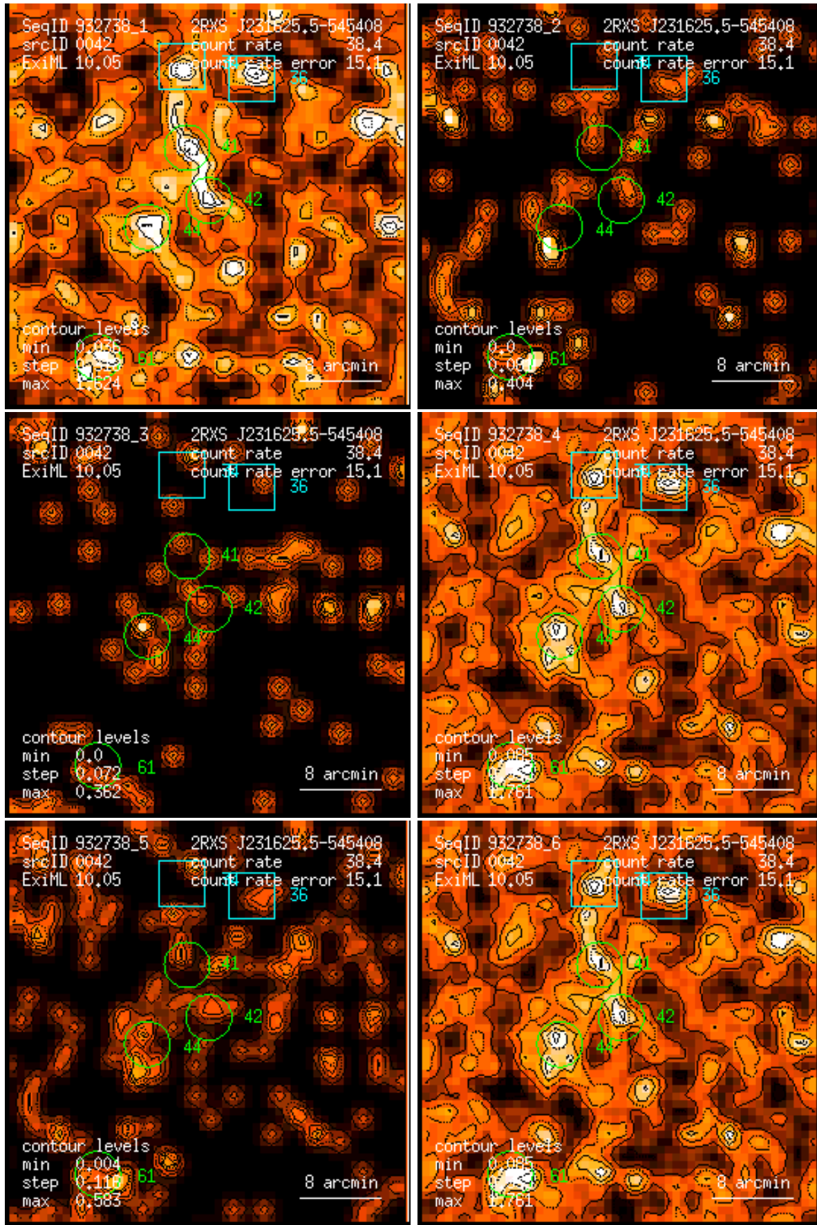
Figure 42: RASS 932738: detection 0042: band rate images, Gaussian filter: (1) PSPC channels 11 – 41, (2) 52 – 90, (3) 91 – 201, (4) 11 – 235, (5) 52 – 201, (6) 11 – 201. Broad band rates in counts/ks. Band rate contour levels in counts/ks/arcmin 2 .
