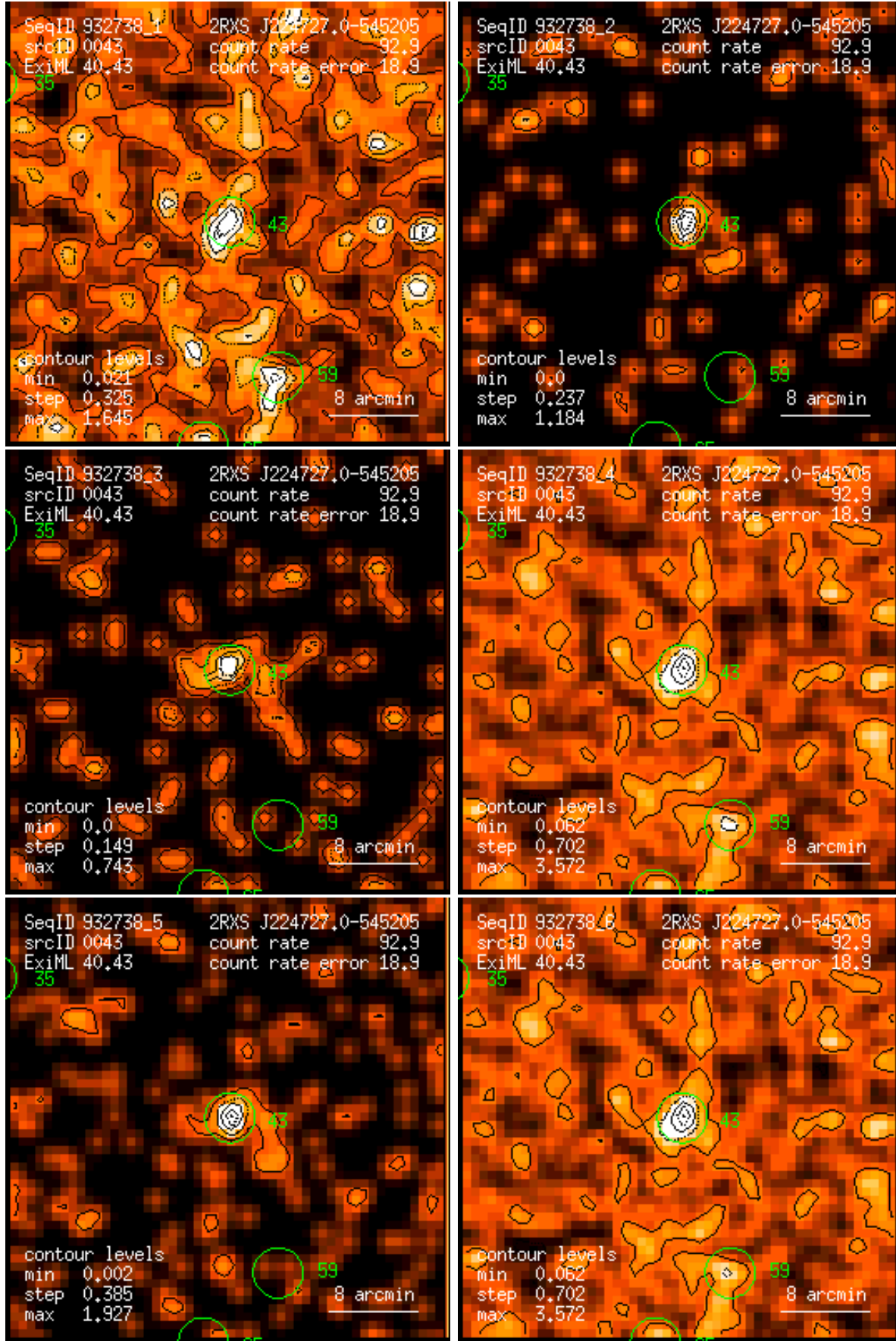
Figure 43: RASS 932738: detection 0043: band rate images, Gaussian filter: (1) PSPC channels 11 – 41, (2) 52 – 90, (3) 91 – 201, (4) 11 – 235, (5) 52 – 201, (6) 11 – 201. Broad band rates in counts/ks. Band rate contour levels in counts/ks/arcmin 2 .
