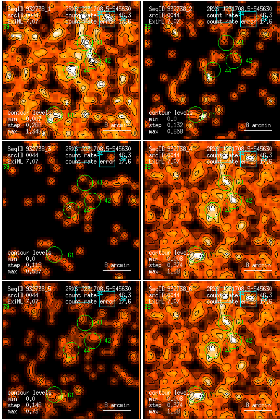
Figure 44: RASS 932738: detection 0044: band rate images, Gaussian filter: (1) PSPC channels 11 – 41, (2) 52 – 90, (3) 91 – 201, (4) 11 – 235, (5) 52 – 201, (6) 11 – 201. Broad band rates in counts/ks. Band rate contour levels in counts/ks/arcmin 2 .
