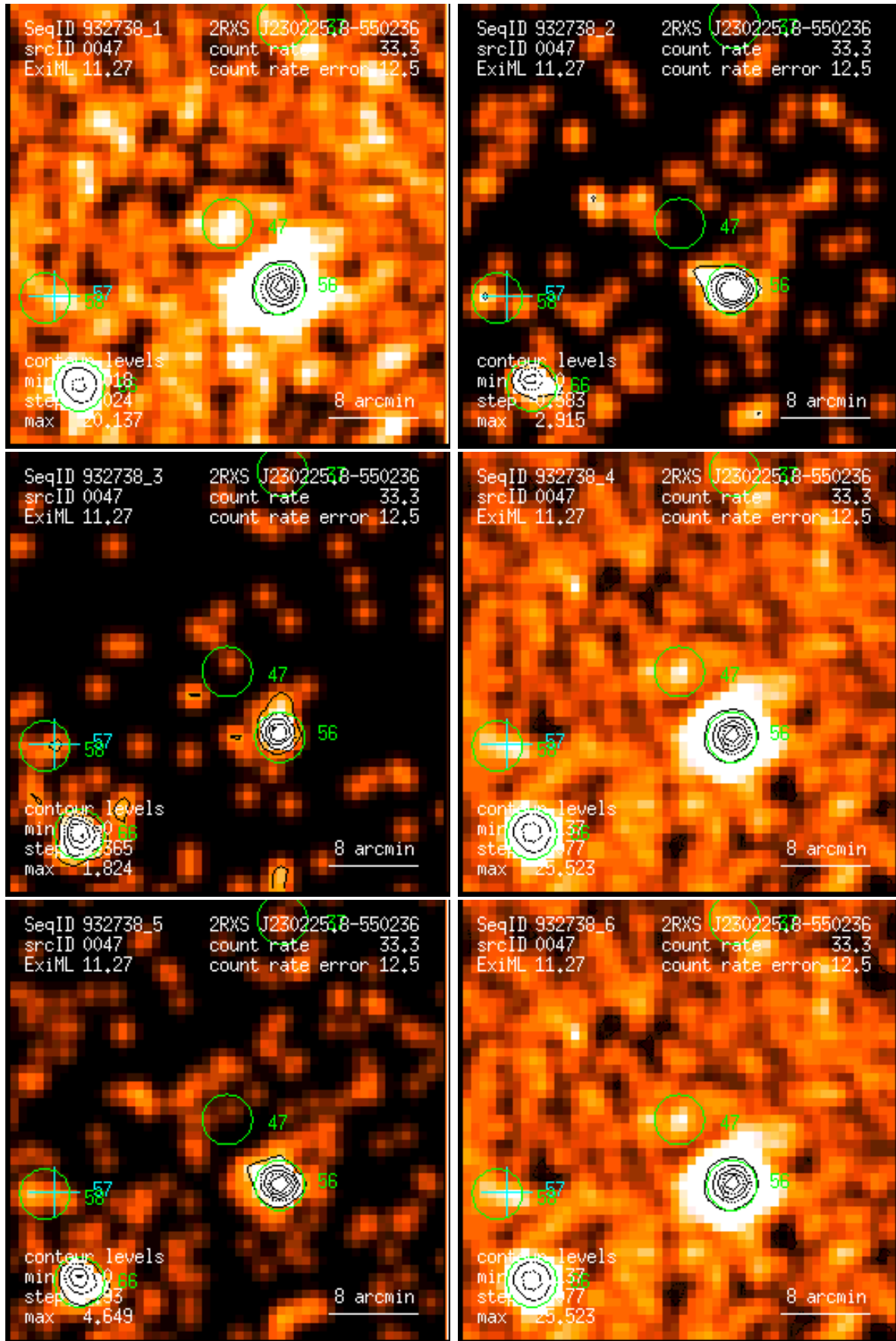
Figure 47: RASS 932738: detection 0047: band rate images, Gaussian filter: (1) PSPC channels 11 – 41, (2) 52 – 90, (3) 91 – 201, (4) 11 – 235, (5) 52 – 201, (6) 11 – 201. Broad band rates in counts/ks. Band rate contour levels in counts/ks/arcmin 2 .
