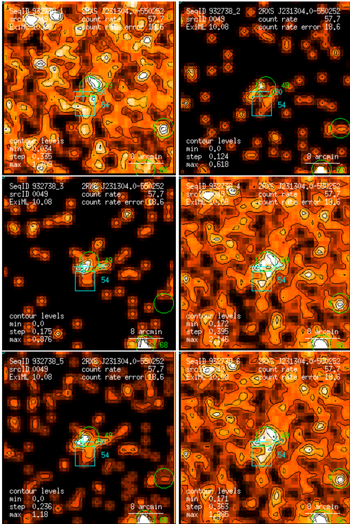
Figure 49: RASS 932738: detection 0049: band rate images, Gaussian filter: (1) PSPC channels 11 – 41, (2) 52 – 90, (3) 91 – 201, (4) 11 – 235, (5) 52 – 201, (6) 11 – 201. Broad band rates in counts/ks. Band rate contour levels in counts/ks/arcmin 2 .
