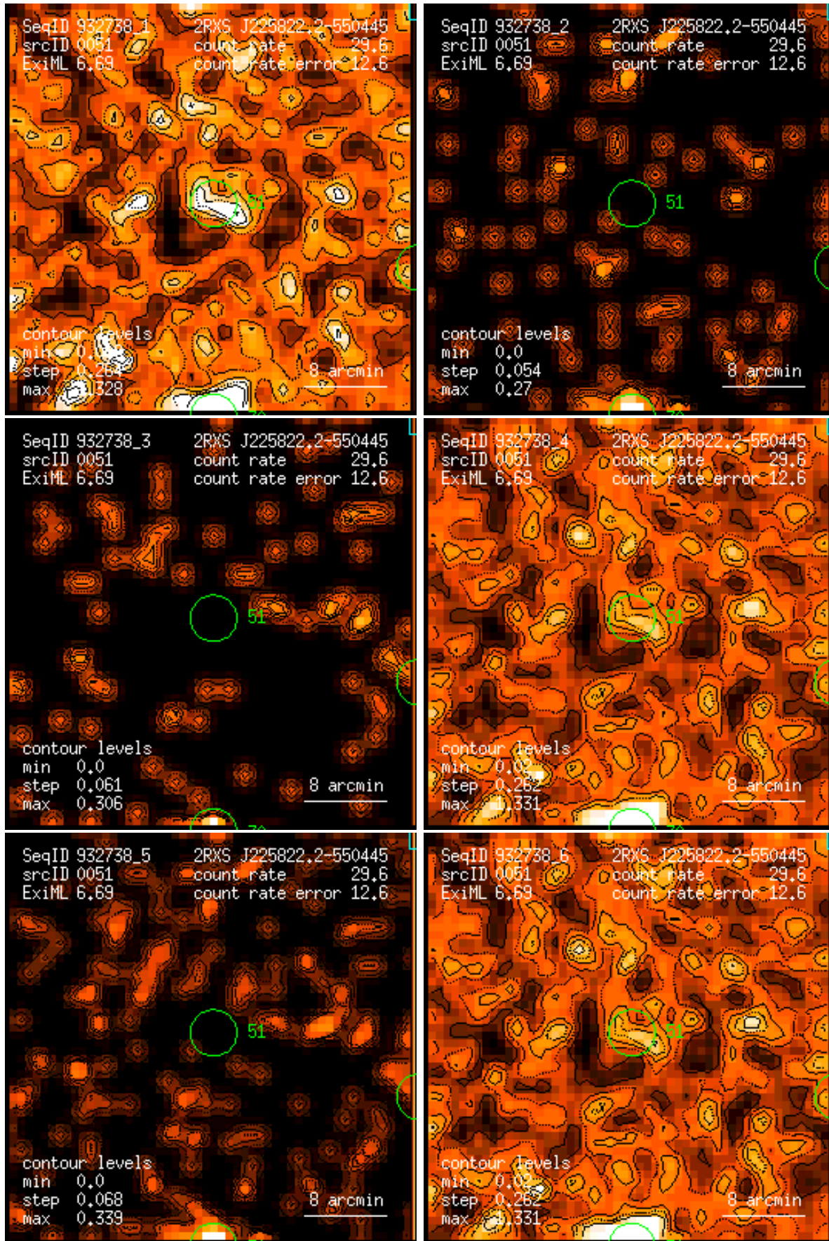
Figure 51: RASS 932738: detection 0051: band rate images, Gaussian filter: (1) PSPC channels 11 – 41, (2) 52 – 90, (3) 91 – 201, (4) 11 – 235, (5) 52 – 201, (6) 11 – 201. Broad band rates in counts/ks. Band rate contour levels in counts/ks/arcmin 2 .
