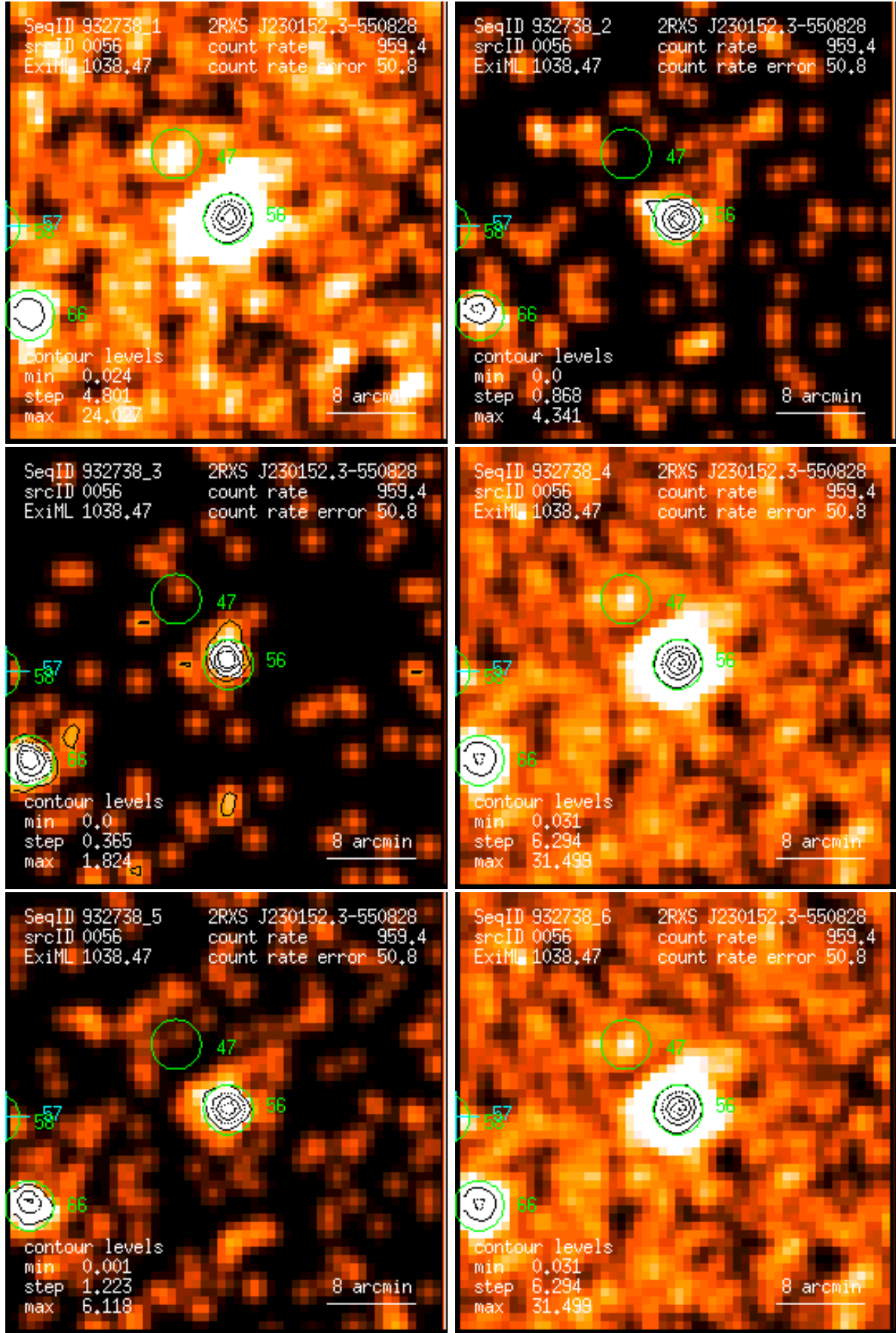
Figure 56: RASS 932738: detection 0056: band rate images, Gaussian filter: (1) PSPC channels 11 – 41, (2) 52 – 90, (3) 91 – 201, (4) 11 – 235, (5) 52 – 201, (6) 11 – 201. Broad band rates in counts/ks. Band rate contour levels in counts/ks/arcmin 2 .
