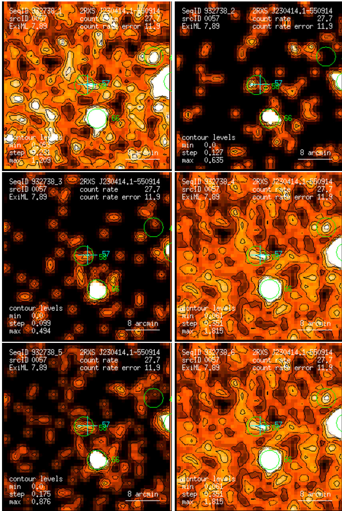
Figure 57: RASS 932738: detection 0057: band rate images, Gaussian filter: (1) PSPC channels 11 – 41, (2) 52 – 90, (3) 91 – 201, (4) 11 – 235, (5) 52 – 201, (6) 11 – 201. Broad band rates in counts/ks. Band rate contour levels in counts/ks/arcmin 2 .
