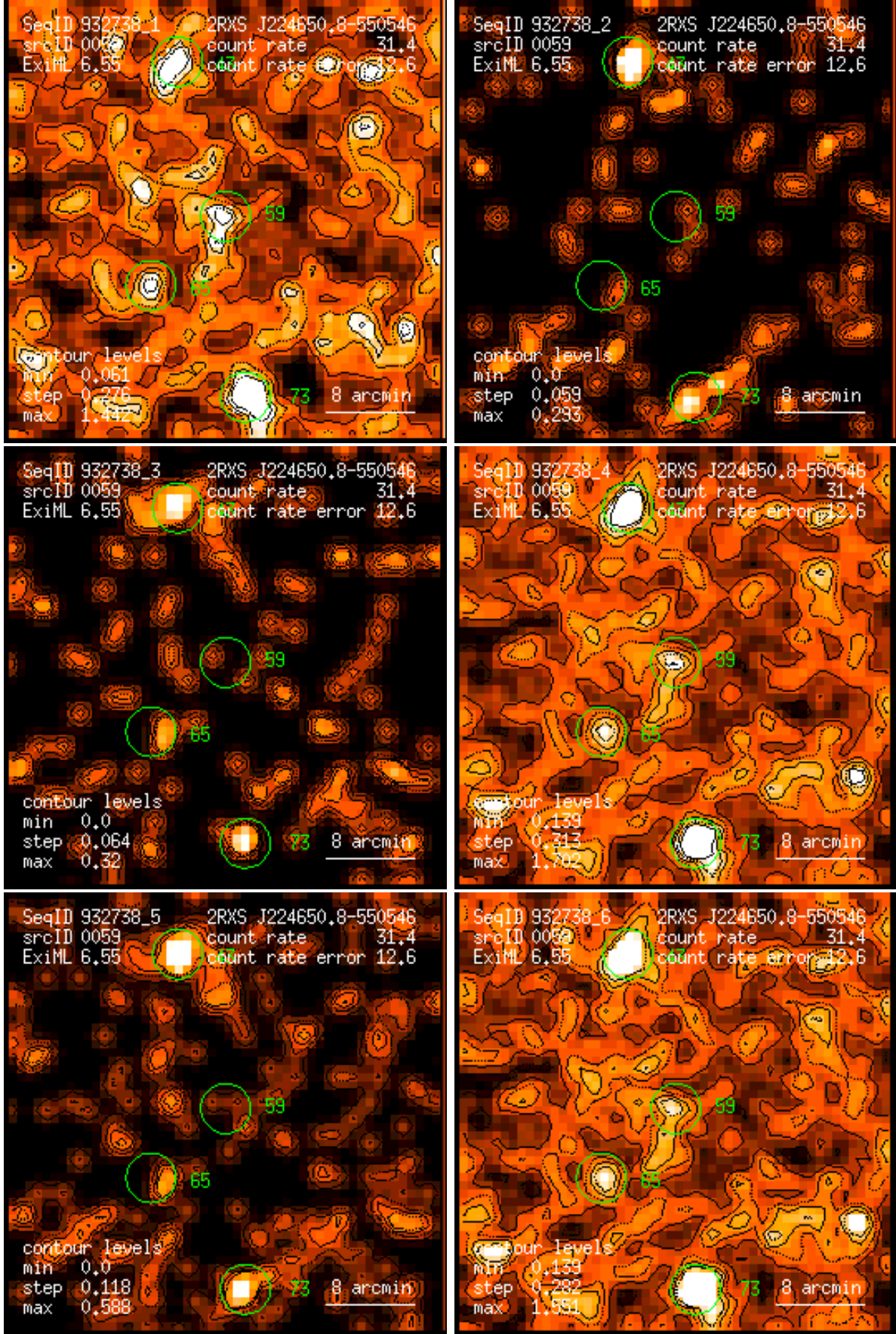
Figure 59: RASS 932738: detection 0059: band rate images, Gaussian filter: (1) PSPC channels 11 – 41, (2) 52 – 90, (3) 91 – 201, (4) 11 – 235, (5) 52 – 201, (6) 11 – 201. Broad band rates in counts/ks. Band rate contour levels in counts/ks/arcmin 2 .
