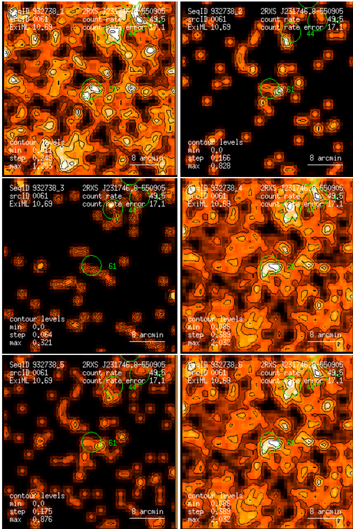
Figure 61: RASS 932738: detection 0061: band rate images, Gaussian filter: (1) PSPC channels 11 – 41, (2) 52 – 90, (3) 91 – 201, (4) 11 – 235, (5) 52 – 201, (6) 11 – 201. Broad band rates in counts/ks. Band rate contour levels in counts/ks/arcmin 2 .
