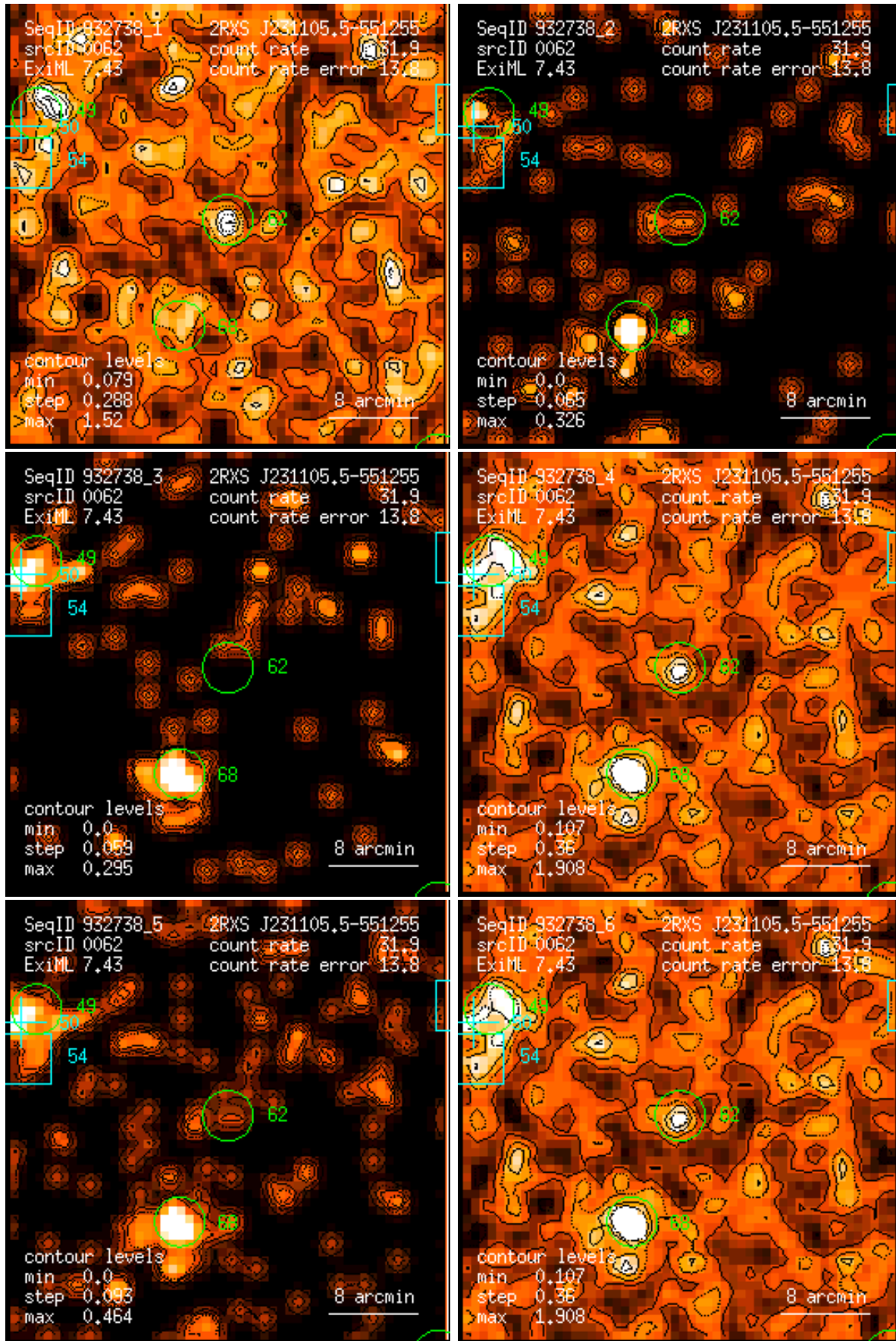
Figure 62: RASS 932738: detection 0062: band rate images, Gaussian filter: (1) PSPC channels 11 – 41, (2) 52 – 90, (3) 91 – 201, (4) 11 – 235, (5) 52 – 201, (6) 11 – 201. Broad band rates in counts/ks. Band rate contour levels in counts/ks/arcmin 2 .
