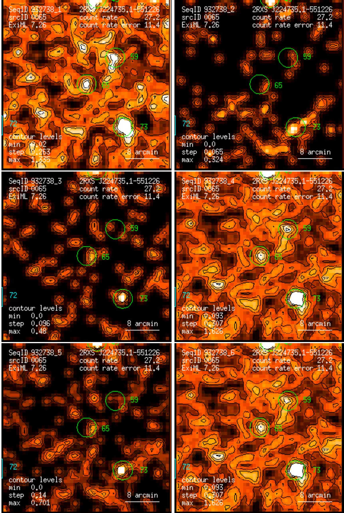
Figure 65: RASS 932738: detection 0065: band rate images, Gaussian filter: (1) PSPC channels 11 – 41, (2) 52 – 90, (3) 91 – 201, (4) 11 – 235, (5) 52 – 201, (6) 11 – 201. Broad band rates in counts/ks. Band rate contour levels in counts/ks/arcmin 2 .
