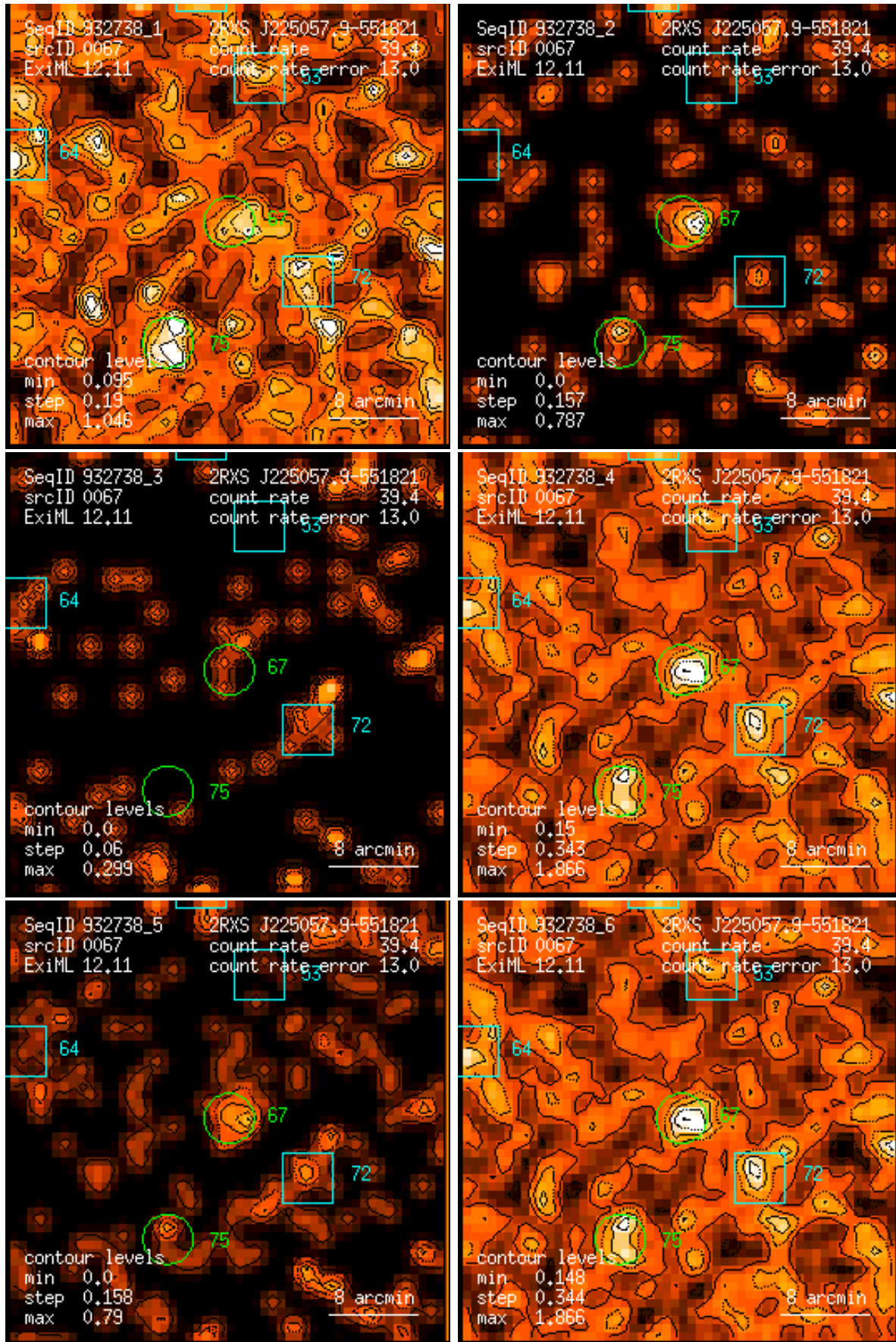
Figure 67: RASS 932738: detection 0067: band rate images, Gaussian filter: (1) PSPC channels 11 – 41, (2) 52 – 90, (3) 91 – 201, (4) 11 – 235, (5) 52 – 201, (6) 11 – 201. Broad band rates in counts/ks. Band rate contour levels in counts/ks/arcmin 2 .
