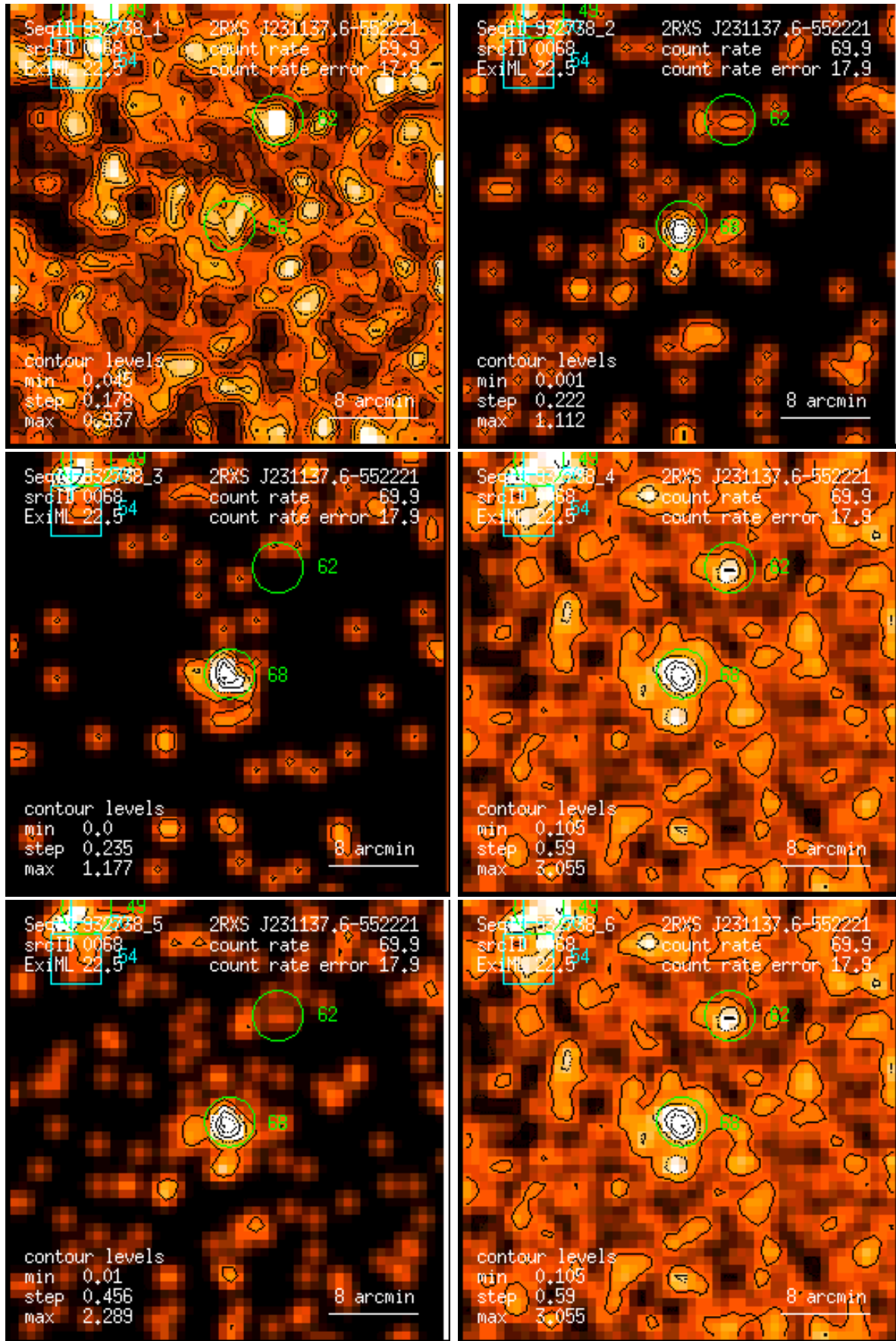
Figure 68: RASS 932738: detection 0068: band rate images, Gaussian filter: (1) PSPC channels 11 – 41, (2) 52 – 90, (3) 91 – 201, (4) 11 – 235, (5) 52 – 201, (6) 11 – 201. Broad band rates in counts/ks. Band rate contour levels in counts/ks/arcmin 2 .
