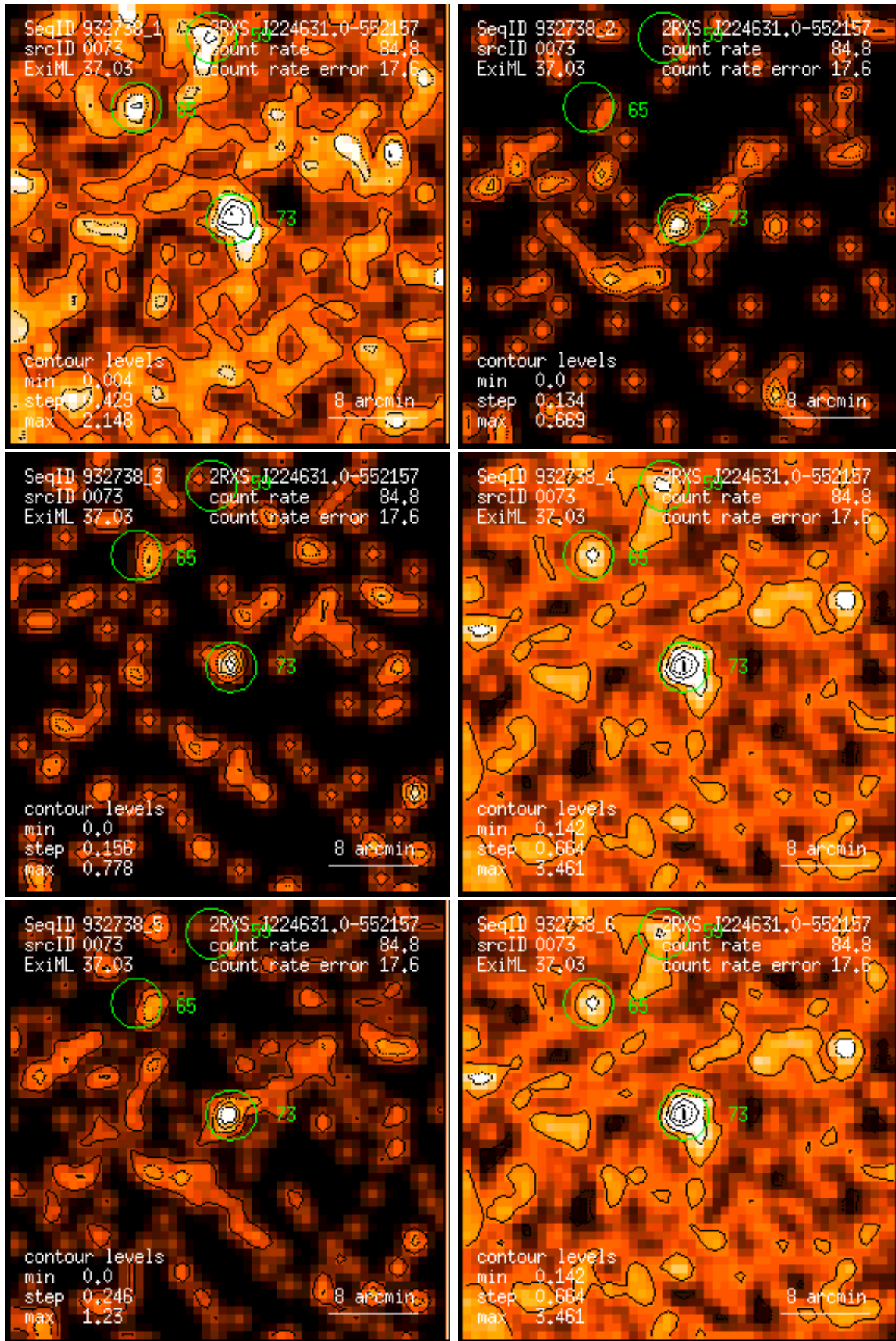
Figure 73: RASS 932738: detection 0073: band rate images, Gaussian filter: (1) PSPC channels 11 – 41, (2) 52 – 90, (3) 91 – 201, (4) 11 – 235, (5) 52 – 201, (6) 11 – 201. Broad band rates in counts/ks. Band rate contour levels in counts/ks/arcmin 2 .
