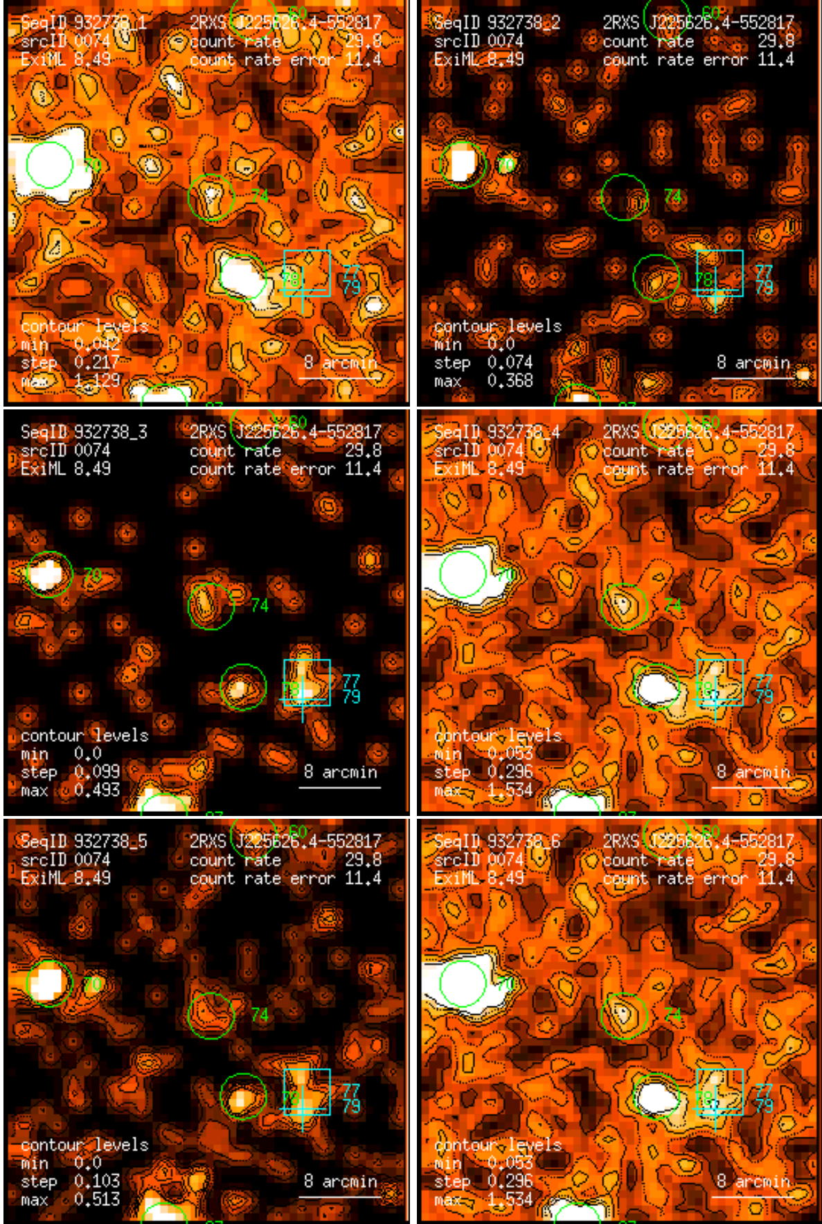
Figure 74: RASS 932738: detection 0074: band rate images, Gaussian filter: (1) PSPC channels 11 – 41, (2) 52 – 90, (3) 91 – 201, (4) 11 – 235, (5) 52 – 201, (6) 11 – 201. Broad band rates in counts/ks. Band rate contour levels in counts/ks/arcmin 2 .
