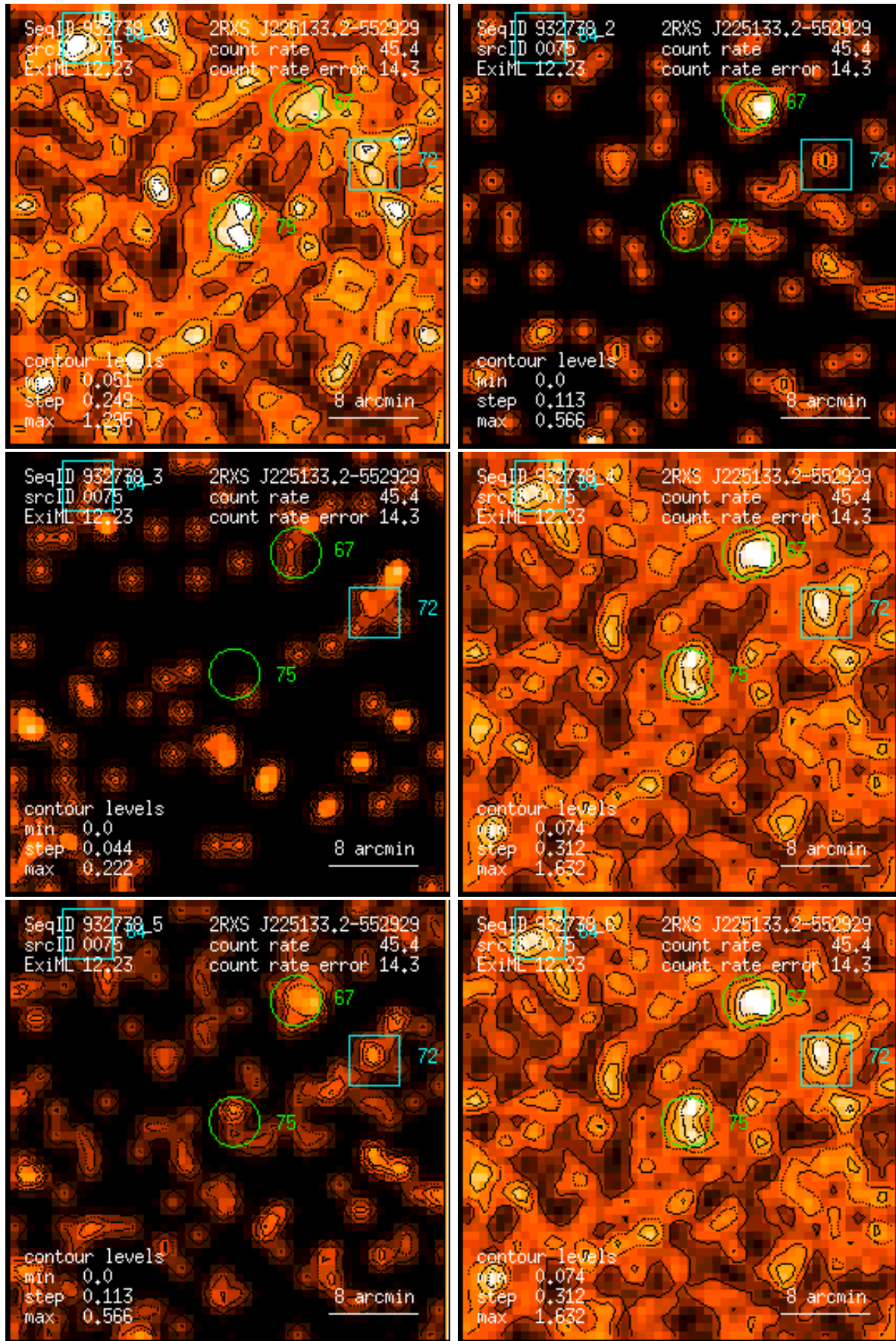
Figure 75: RASS 932738: detection 0075: band rate images, Gaussian filter: (1) PSPC channels 11 – 41, (2) 52 – 90, (3) 91 – 201, (4) 11 – 235, (5) 52 – 201, (6) 11 – 201. Broad band rates in counts/ks. Band rate contour levels in counts/ks/arcmin 2 .
